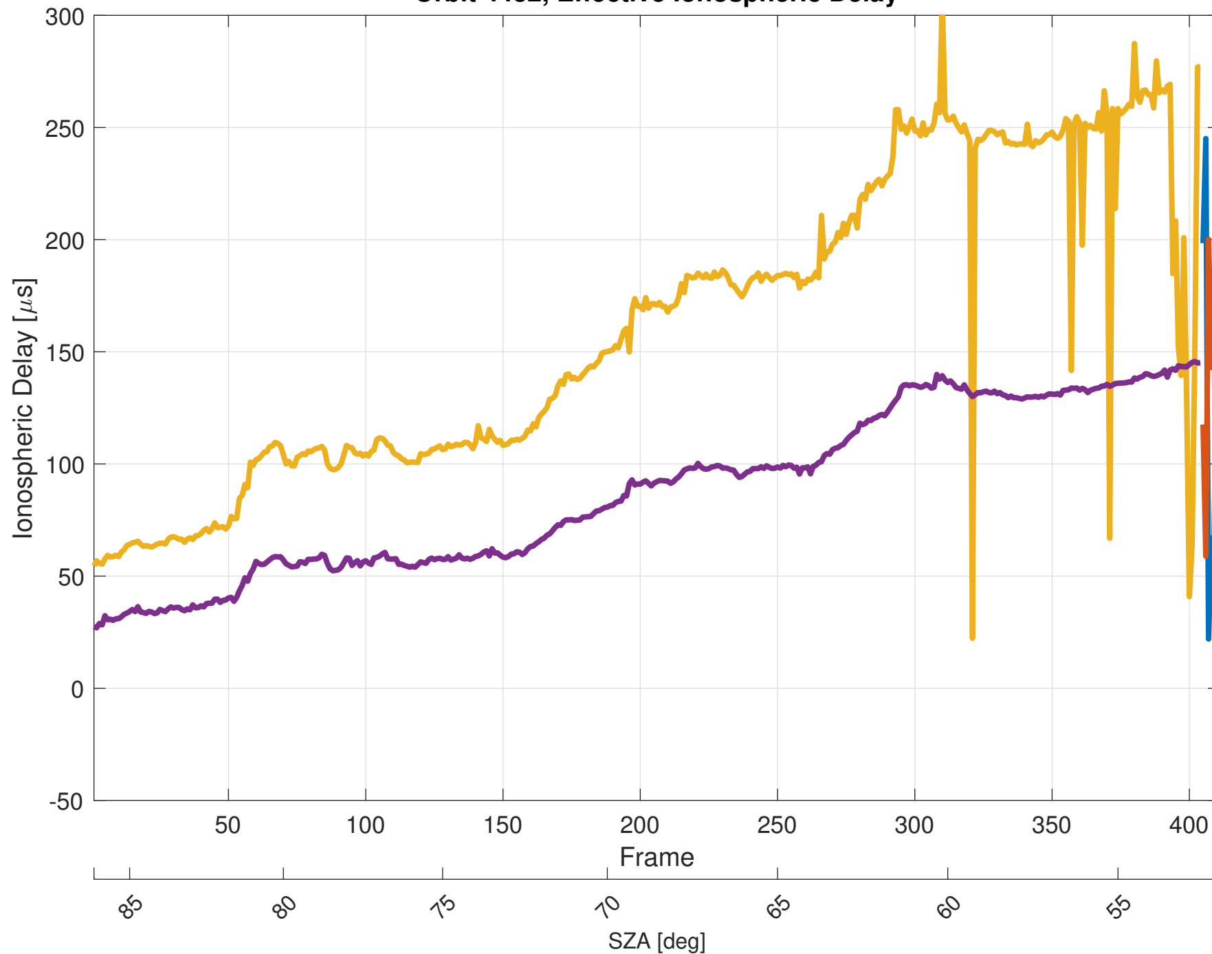
Orbit 4432, Effective Ionospheric Delay
