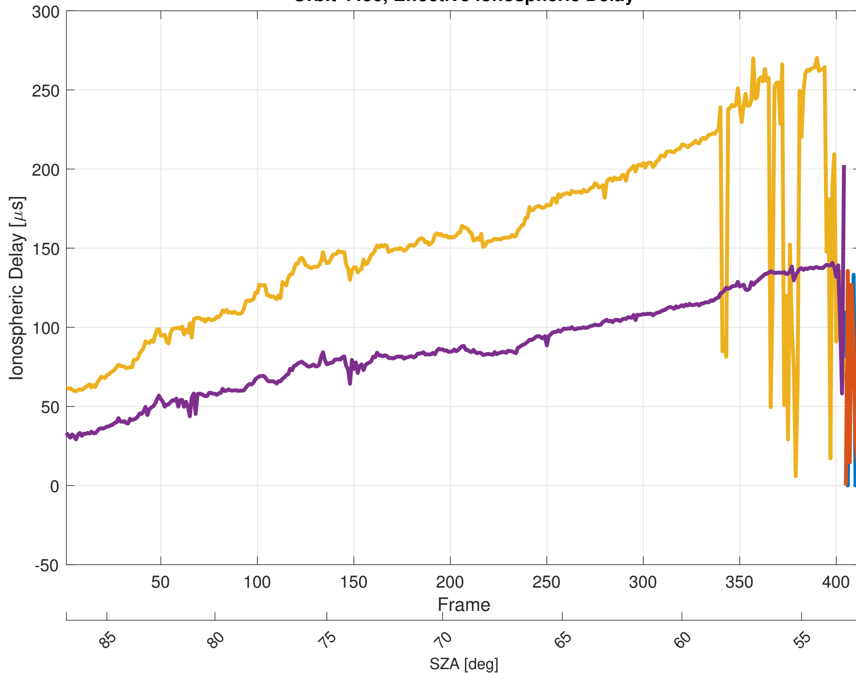
Orbit 4436, Effective Ionospheric Delay
