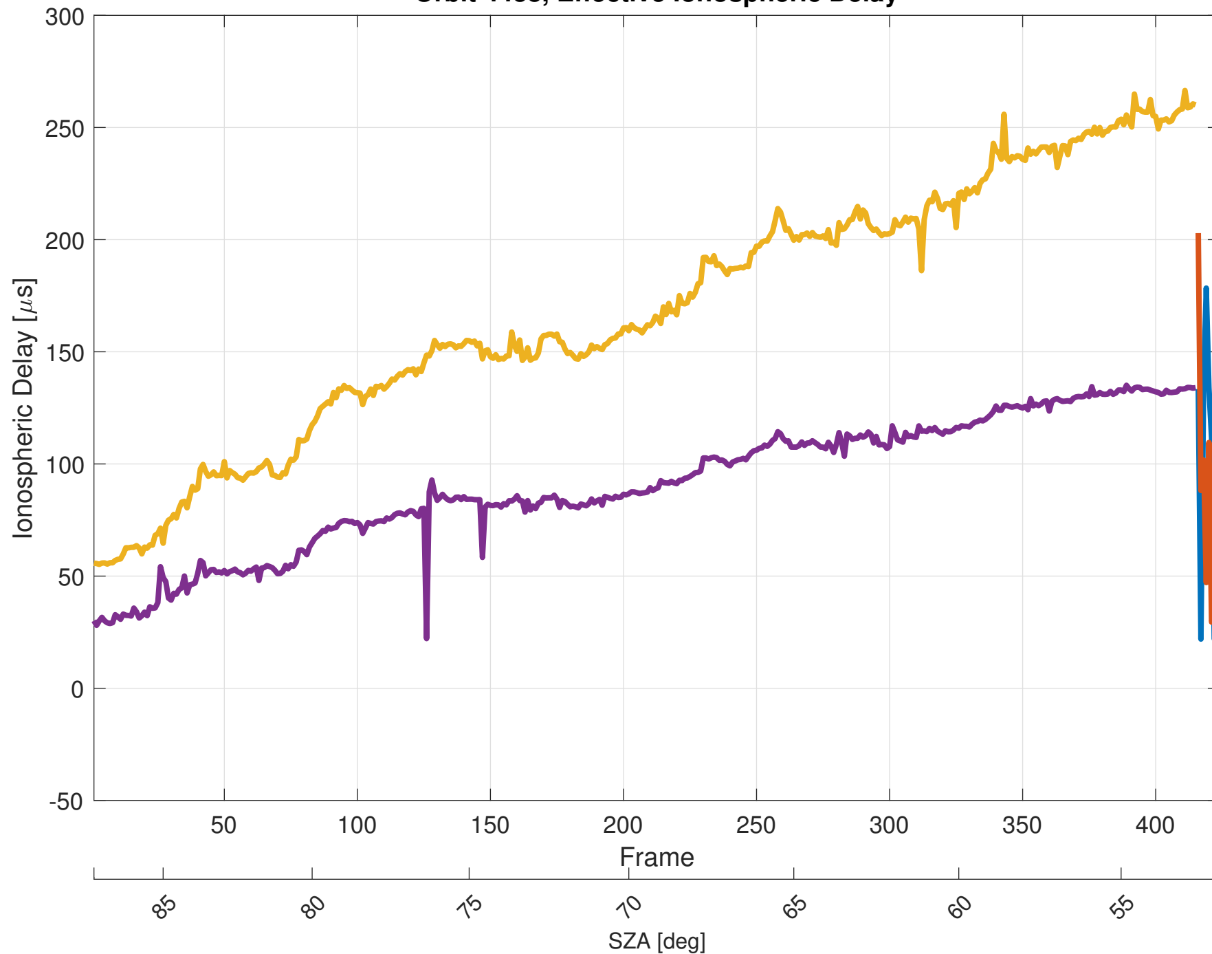
Orbit 4438, Effective Ionospheric Delay
