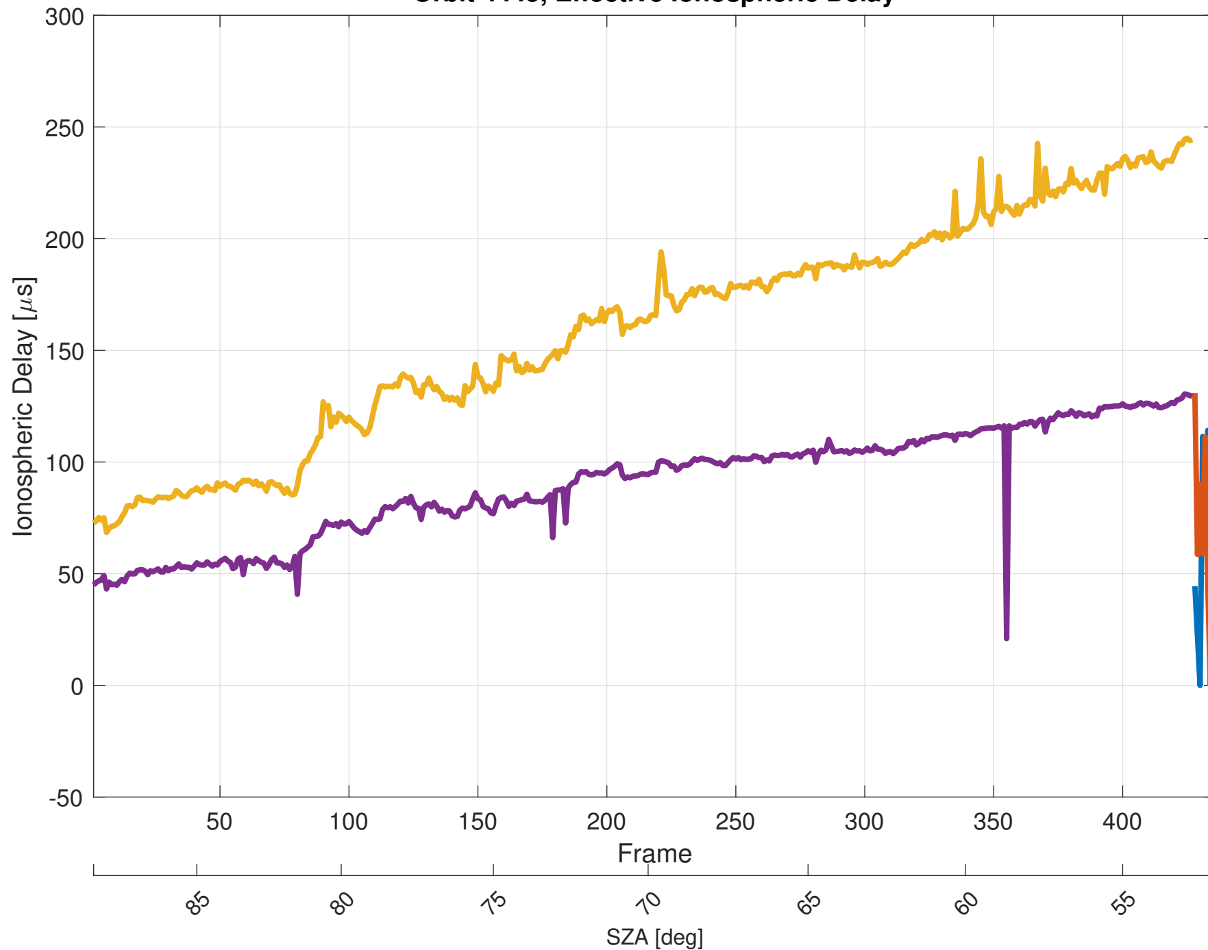
Orbit 4445, Effective Ionospheric Delay
