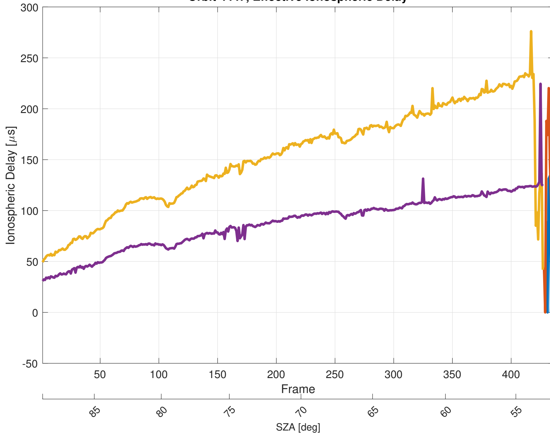
Orbit 4447, Effective Ionospheric Delay
