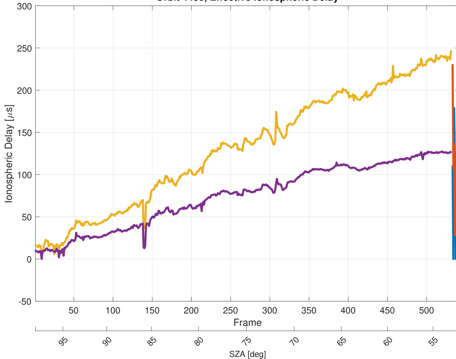
Orbit 4496, Effective Ionospheric Delay
