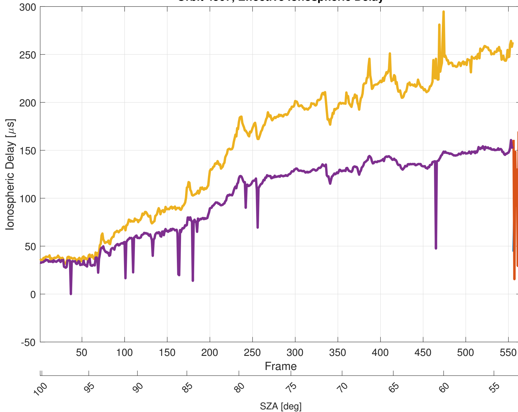
Orbit 4507, Effective Ionospheric Delay
