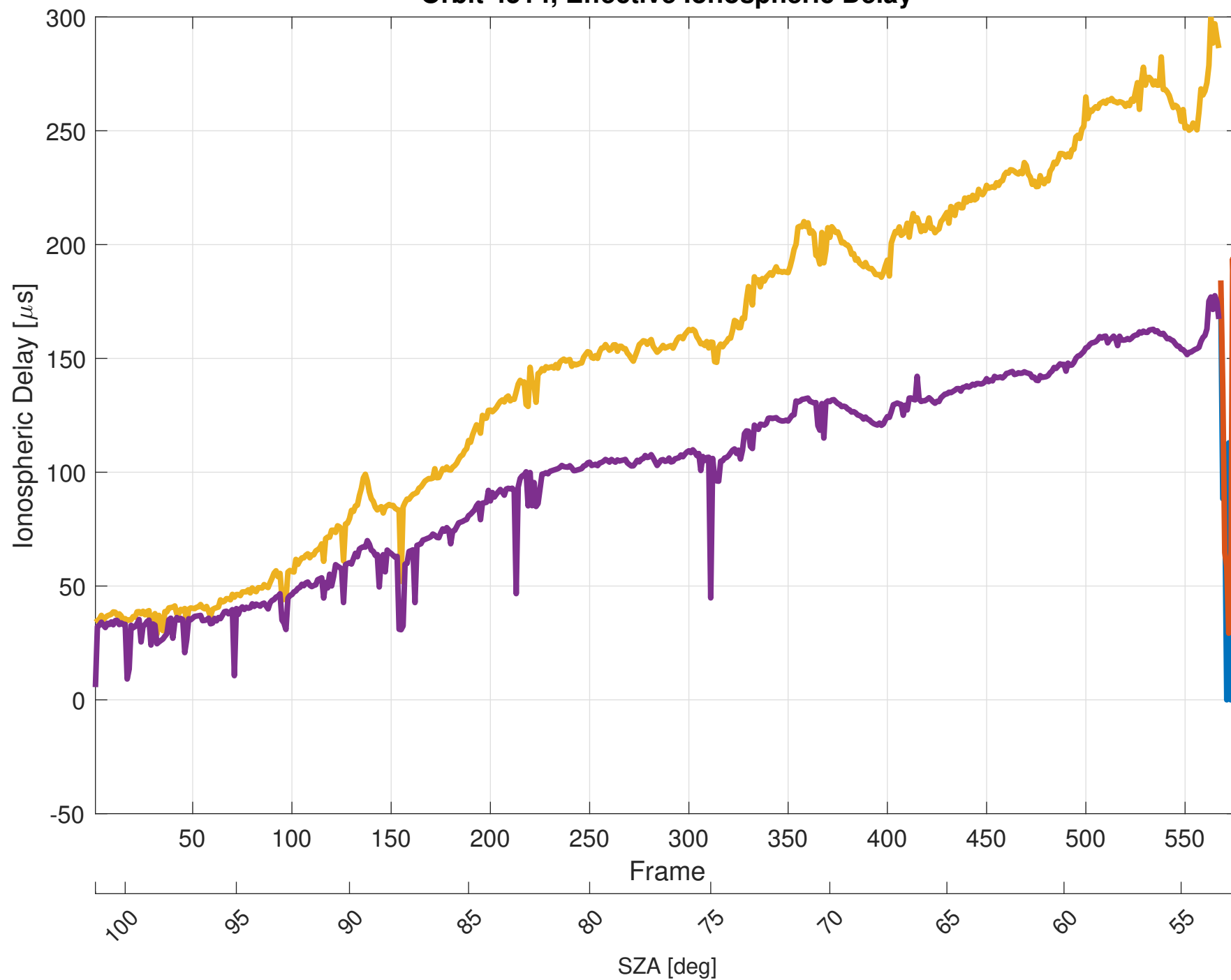
Orbit 4514, Effective Ionospheric Delay
