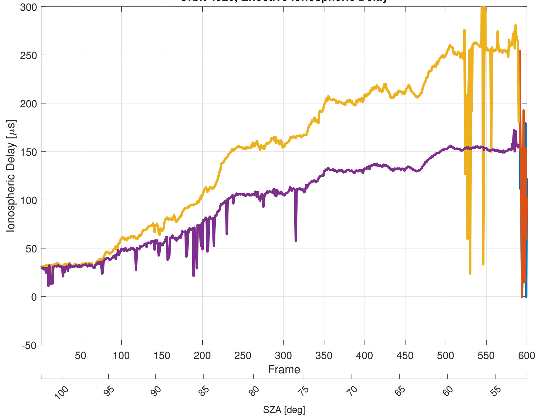
Orbit 4520, Effective Ionospheric Delay
