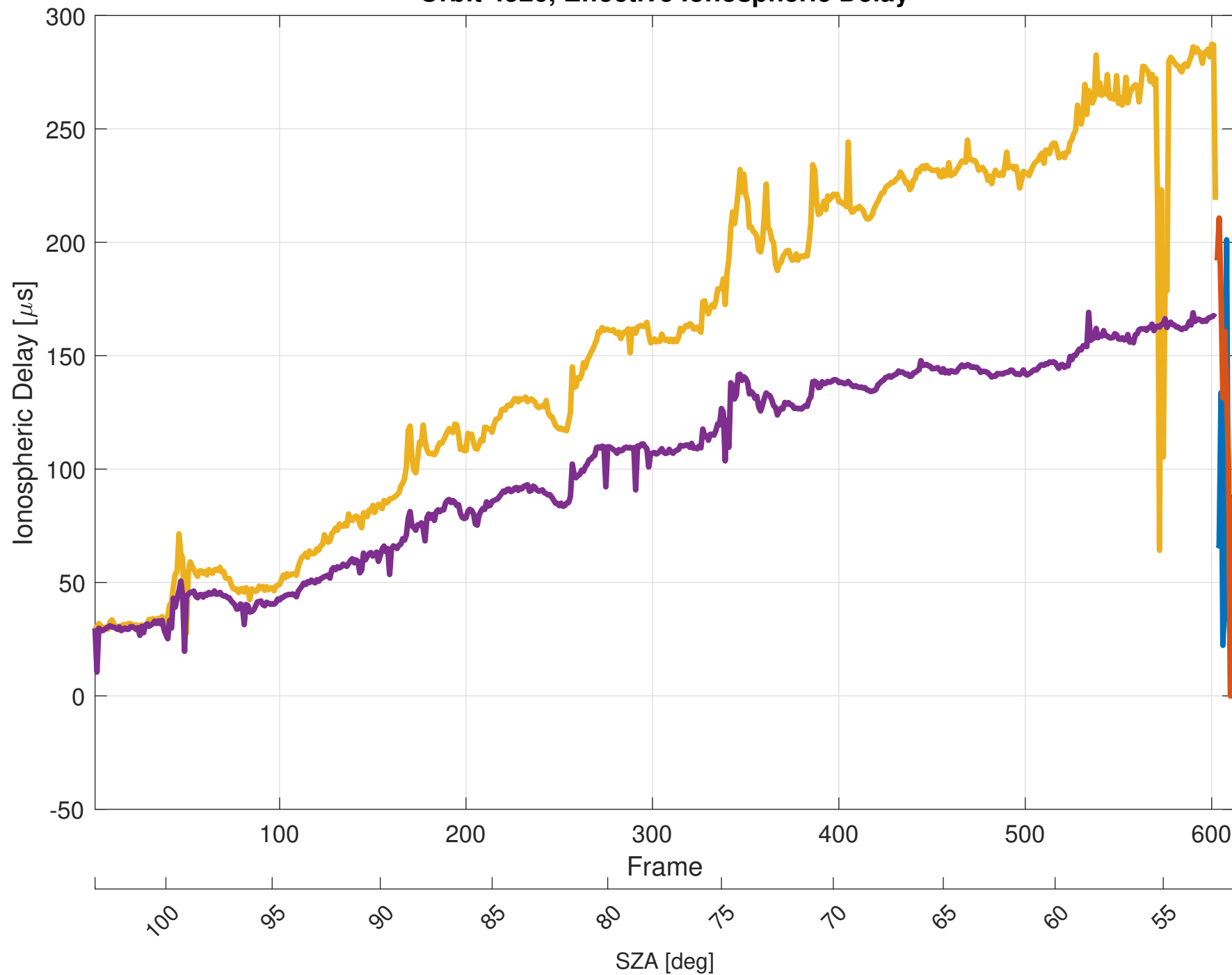
Orbit 4526, Effective Ionospheric Delay
