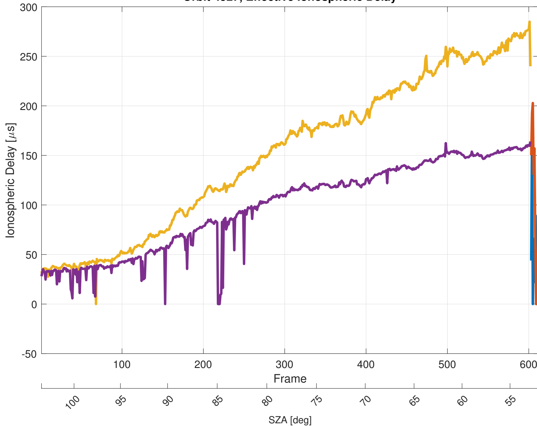
Orbit 4527, Effective Ionospheric Delay
