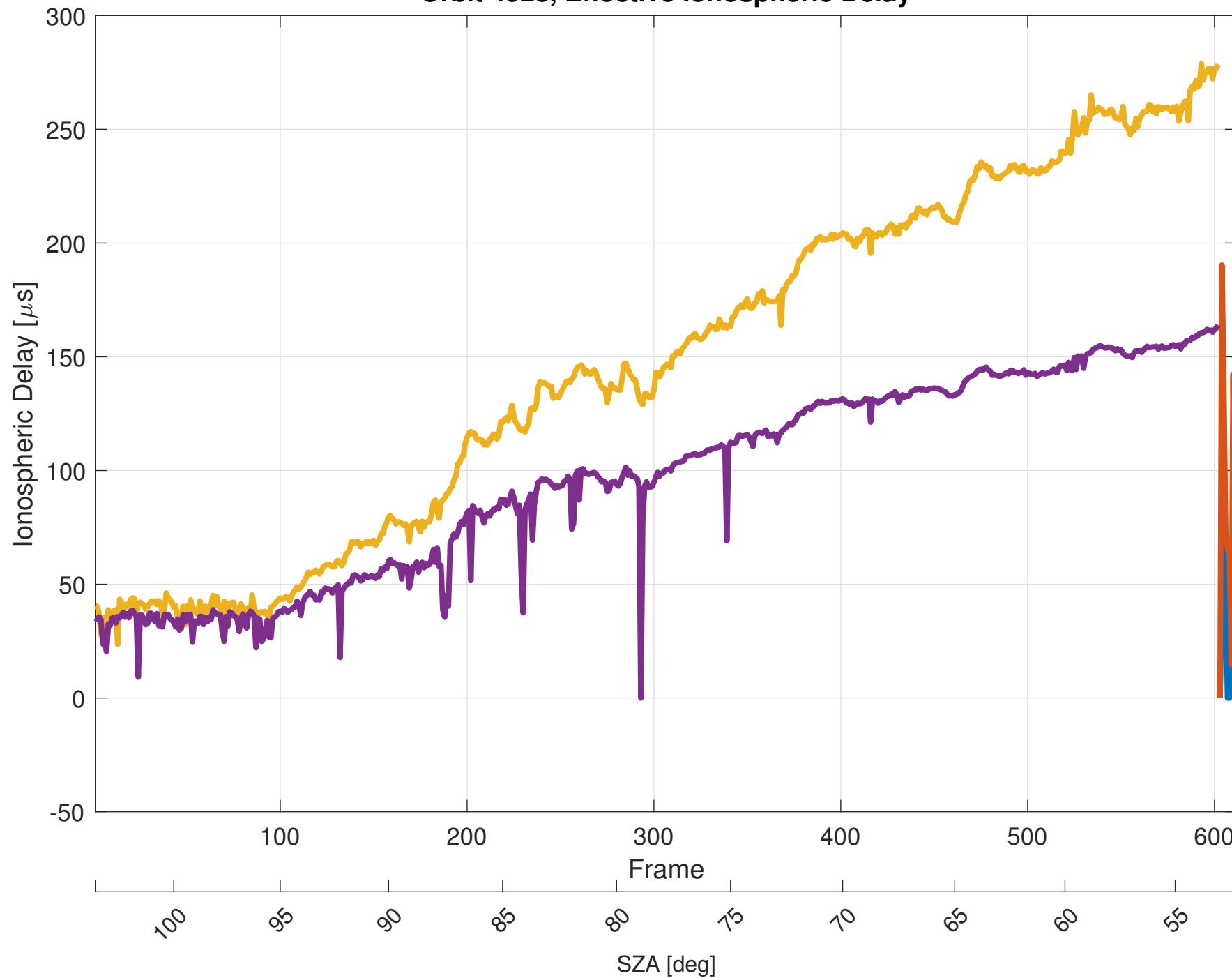
Orbit 4528, Effective Ionospheric Delay
