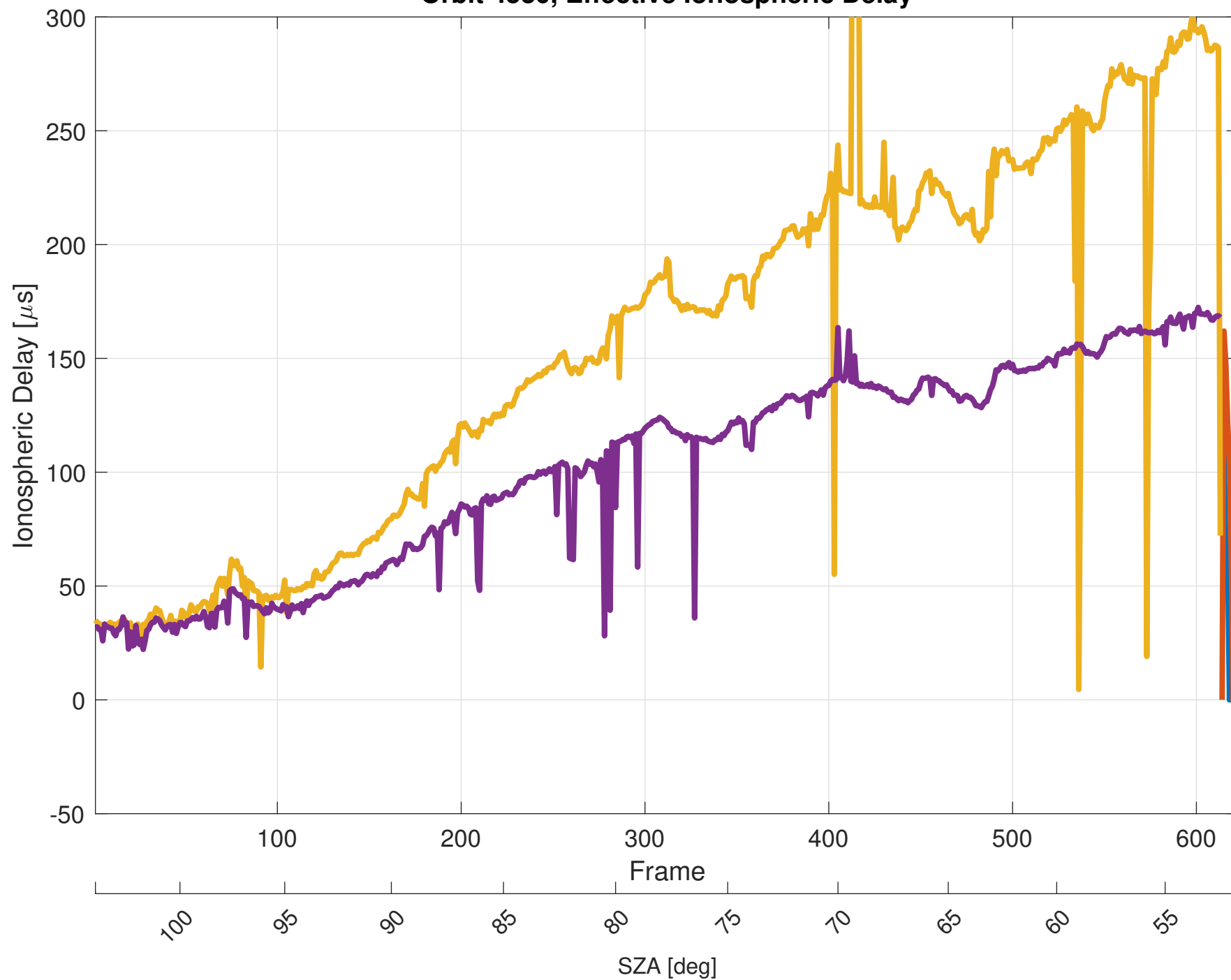
Orbit 4530, Effective Ionospheric Delay
