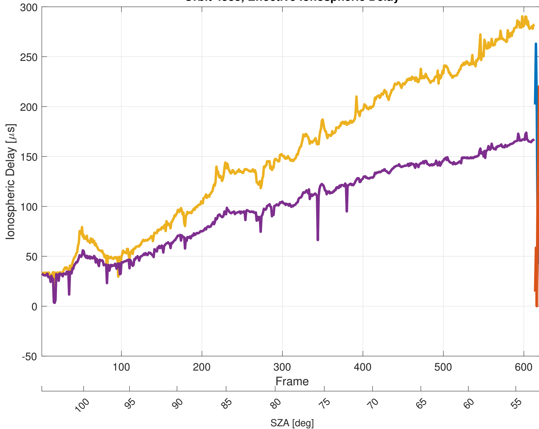
Orbit 4533, Effective Ionospheric Delay
