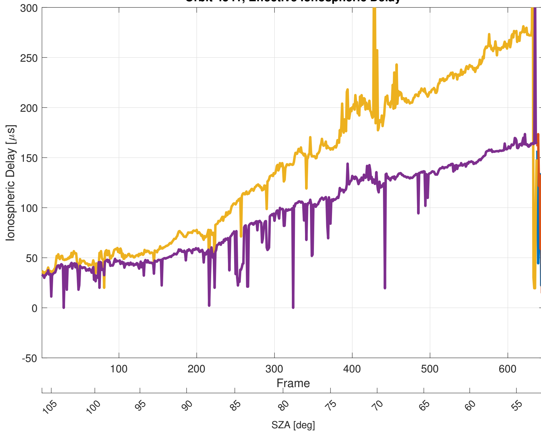
Orbit 4541, Effective Ionospheric Delay
