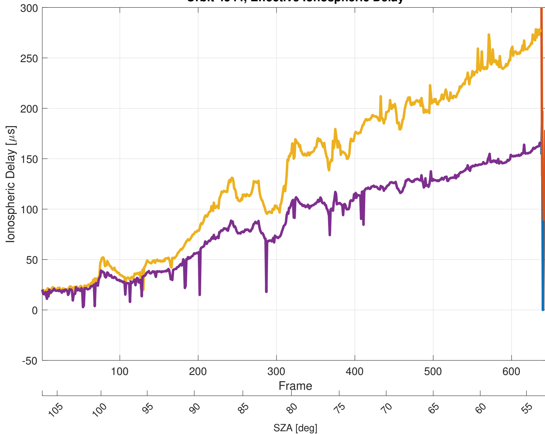
Orbit 4544, Effective Ionospheric Delay
