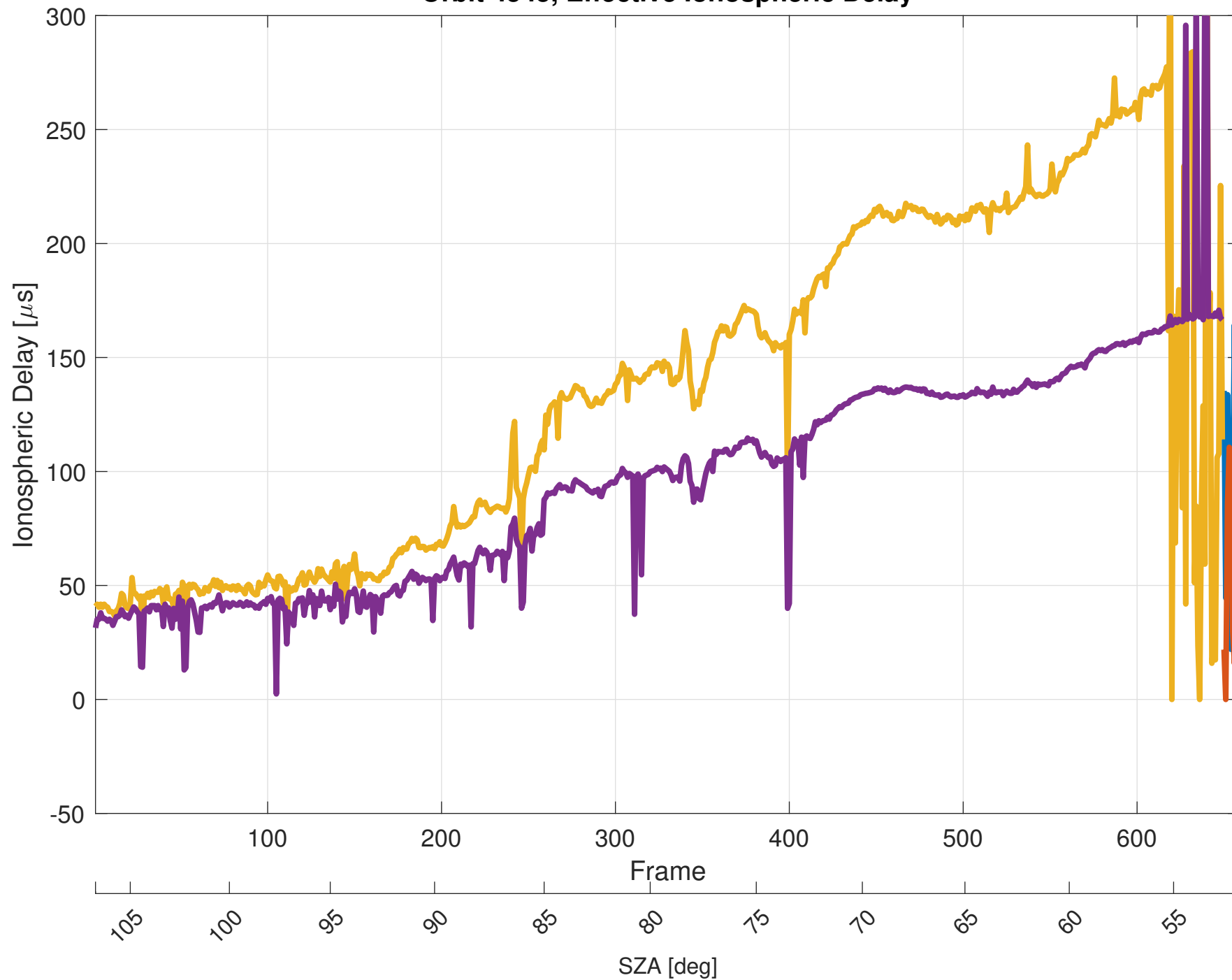
Orbit 4545, Effective Ionospheric Delay
