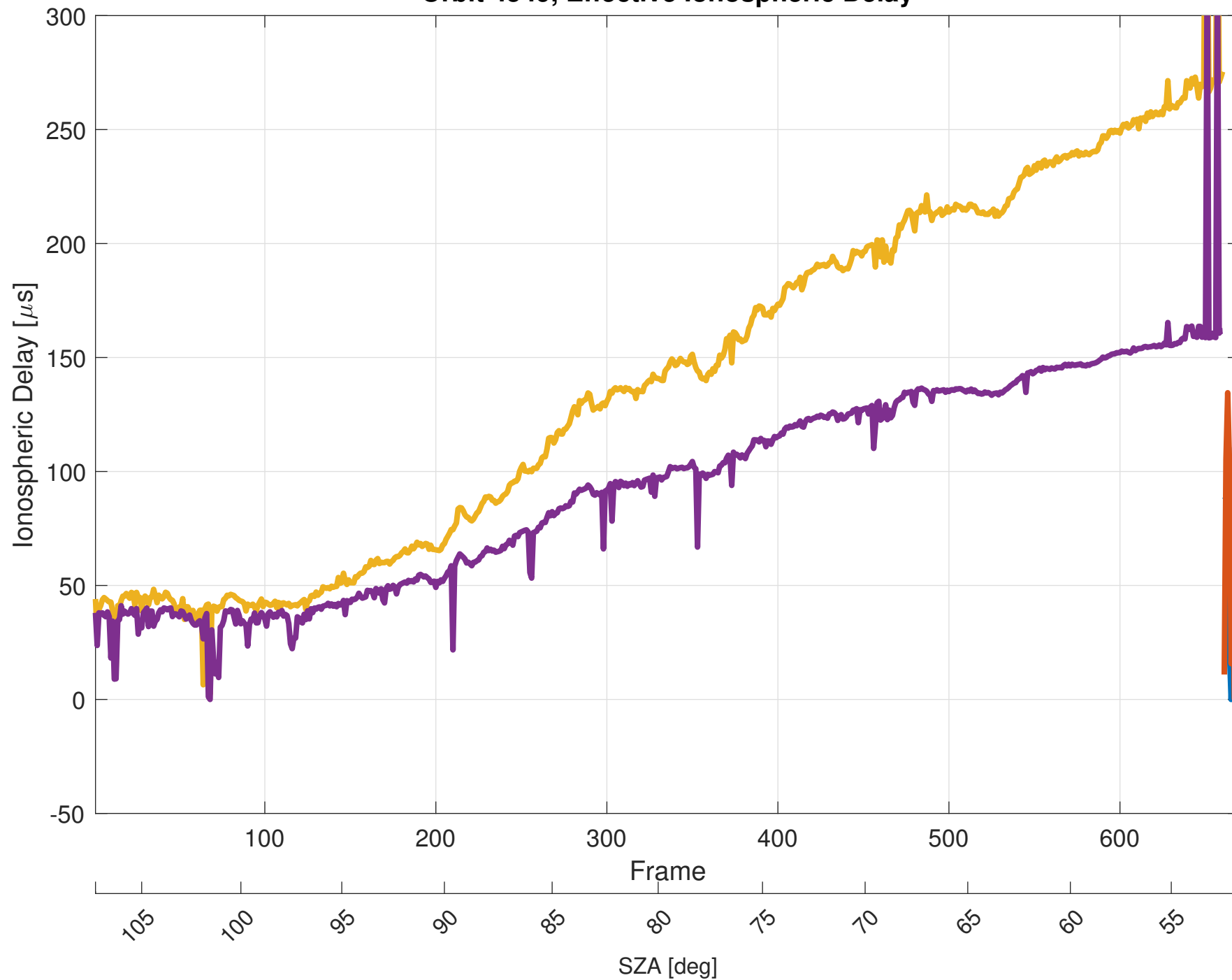
Orbit 4549, Effective Ionospheric Delay
