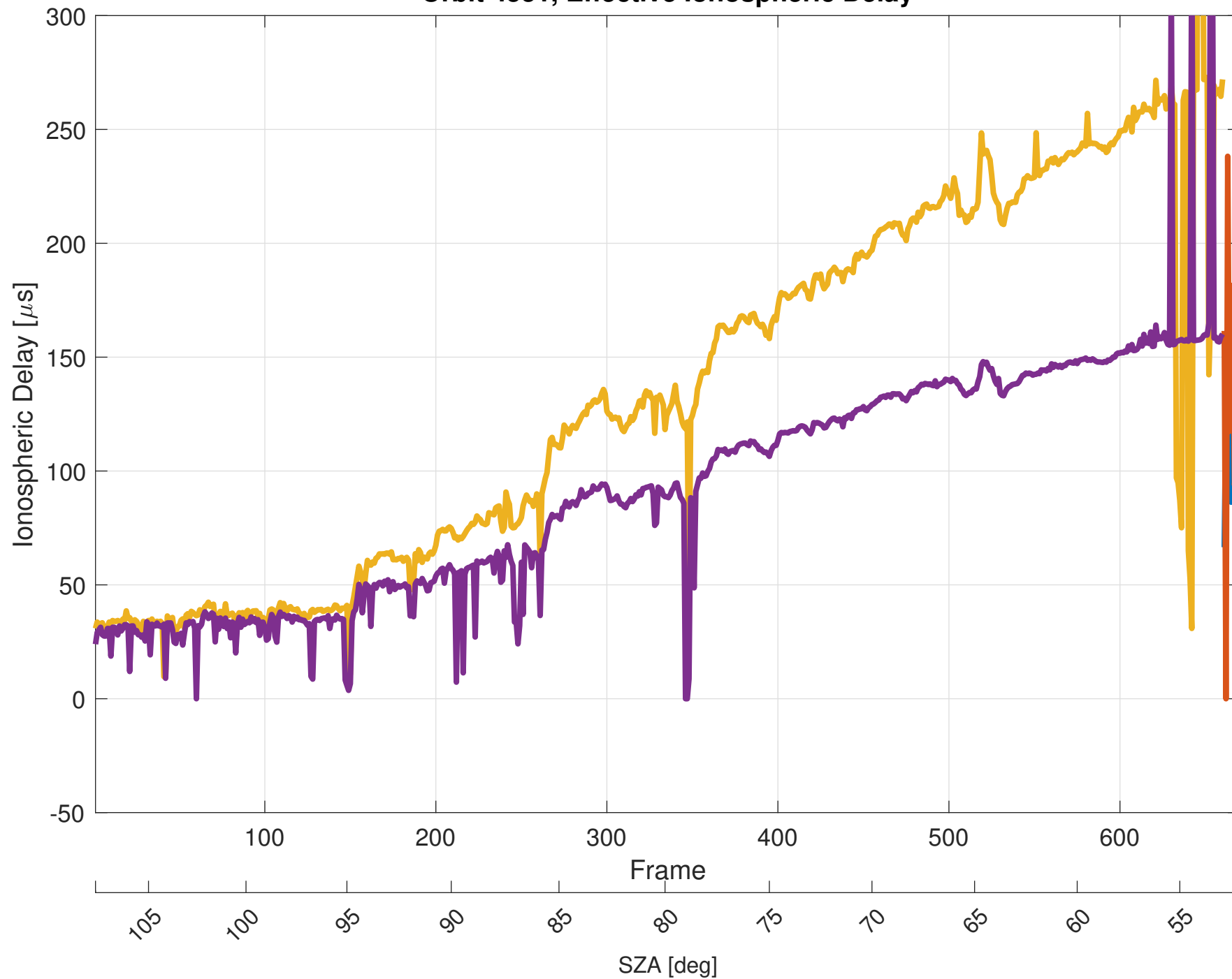
Orbit 4551, Effective Ionospheric Delay
