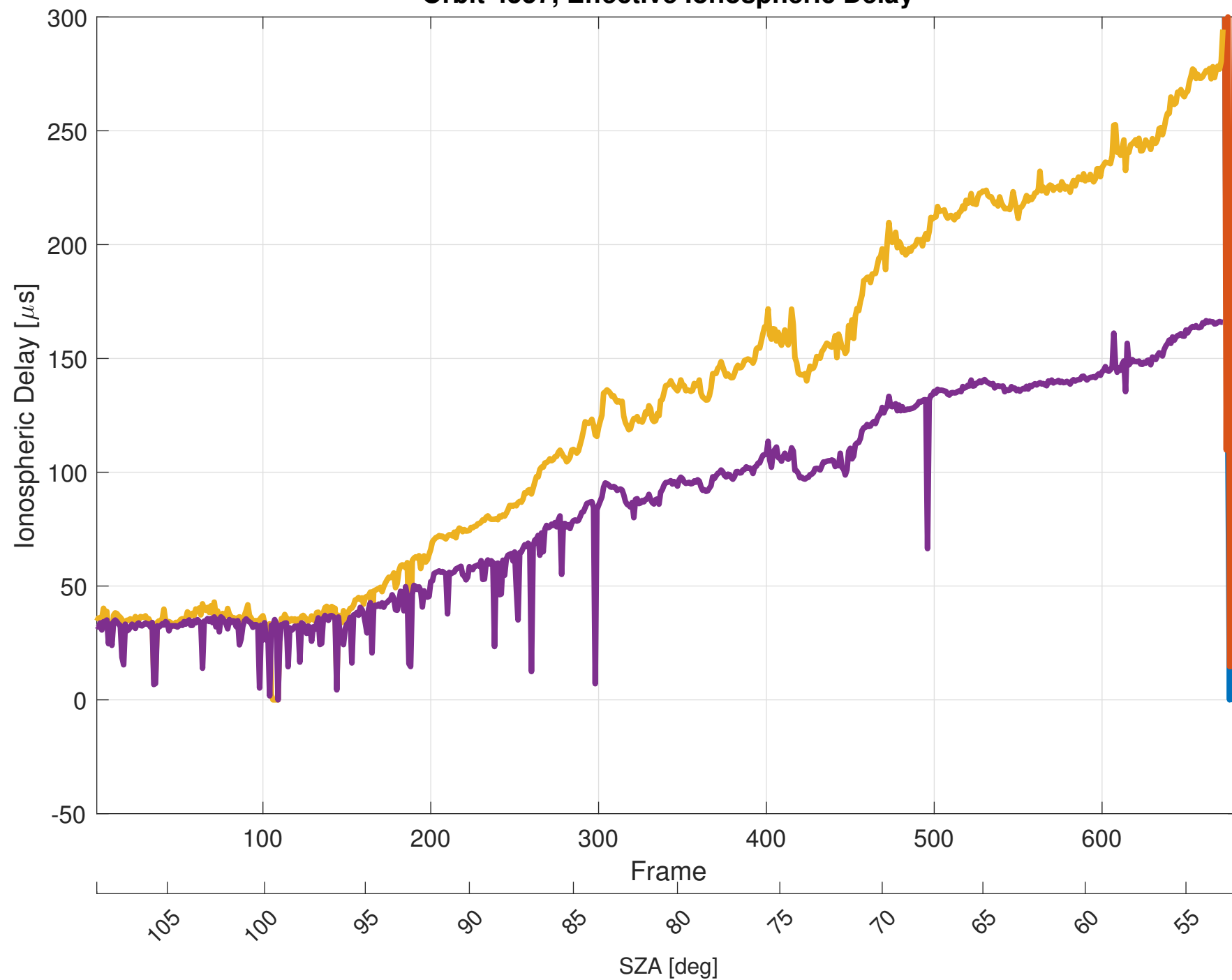
Orbit 4557, Effective Ionospheric Delay
