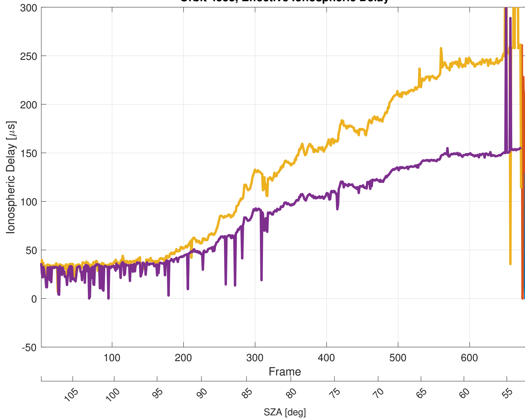
Orbit 4558, Effective Ionospheric Delay
