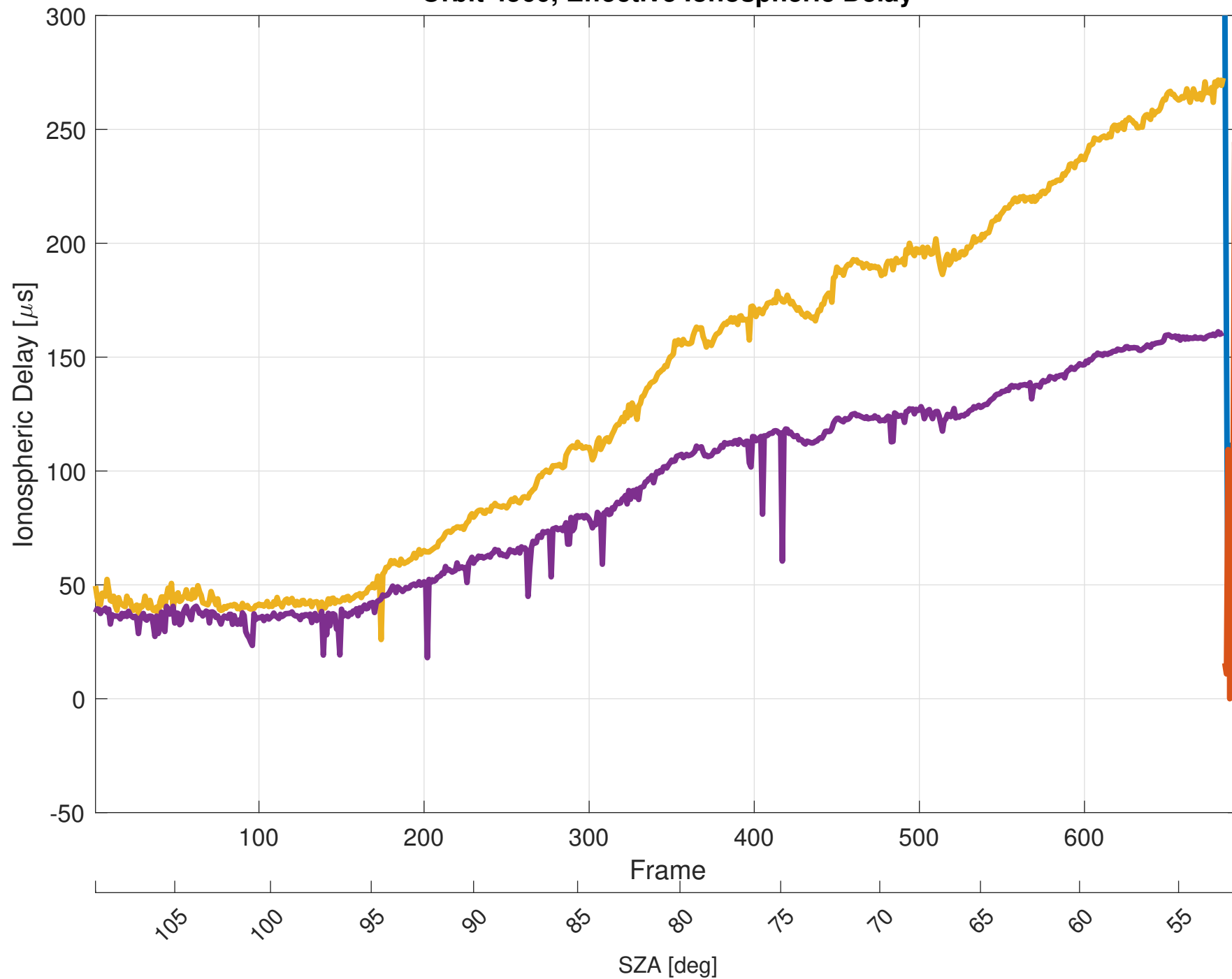
Orbit 4560, Effective Ionospheric Delay
