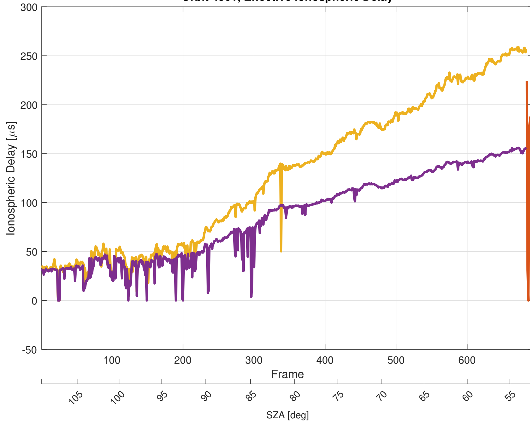
Orbit 4561, Effective Ionospheric Delay
