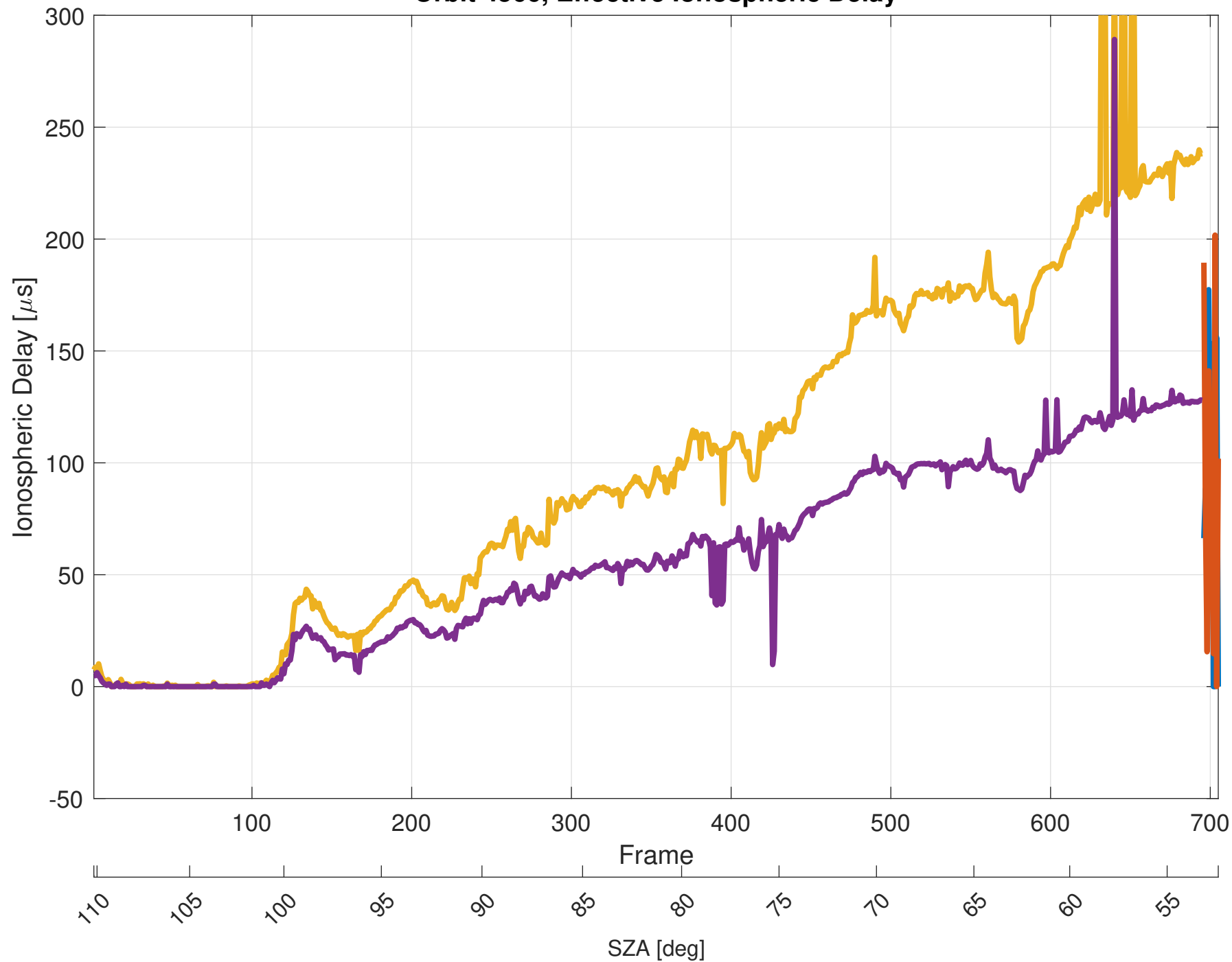
Orbit 4566, Effective Ionospheric Delay
