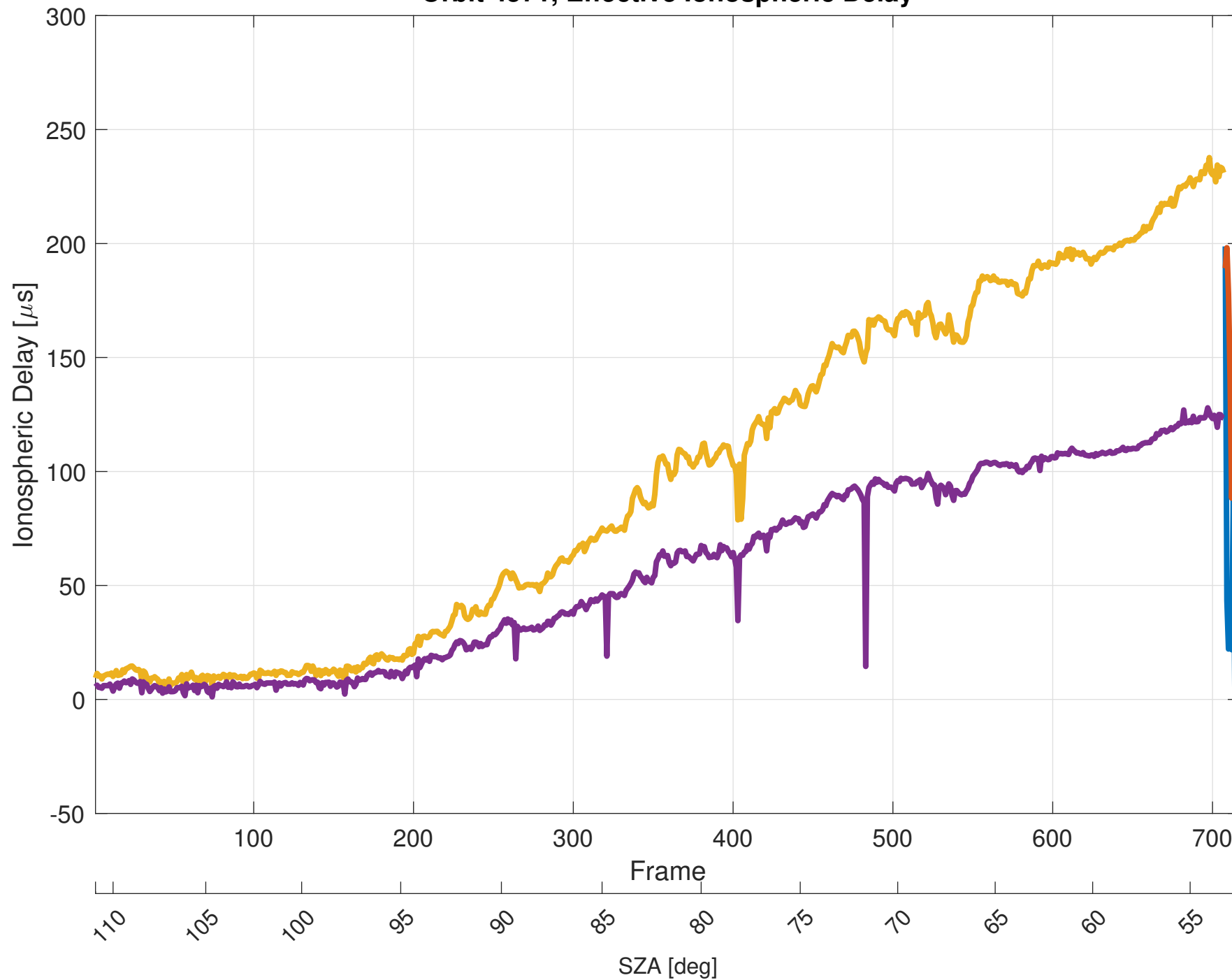
Orbit 4571, Effective Ionospheric Delay
