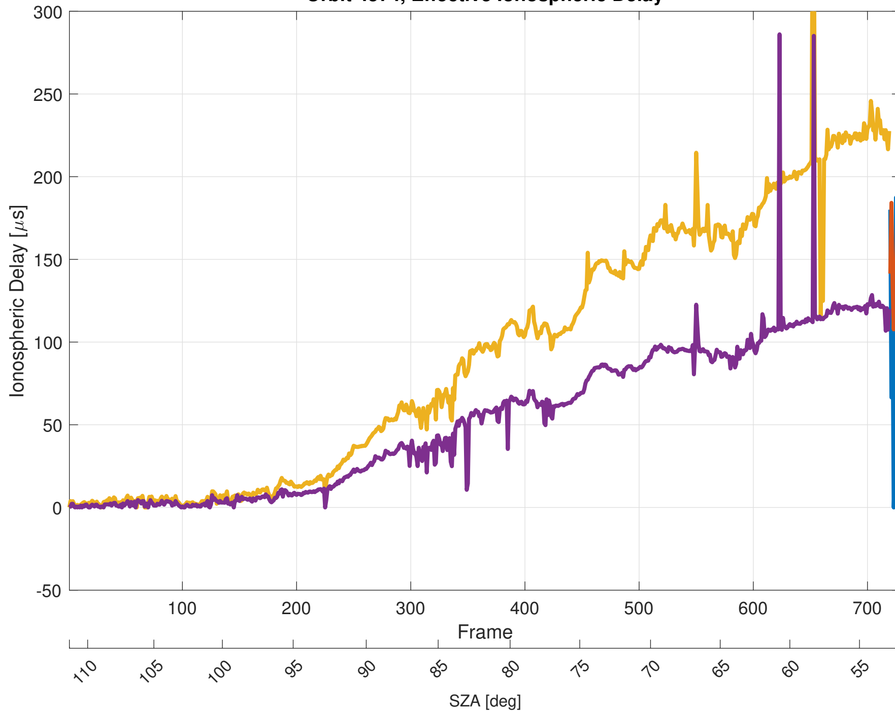
Orbit 4574, Effective Ionospheric Delay
