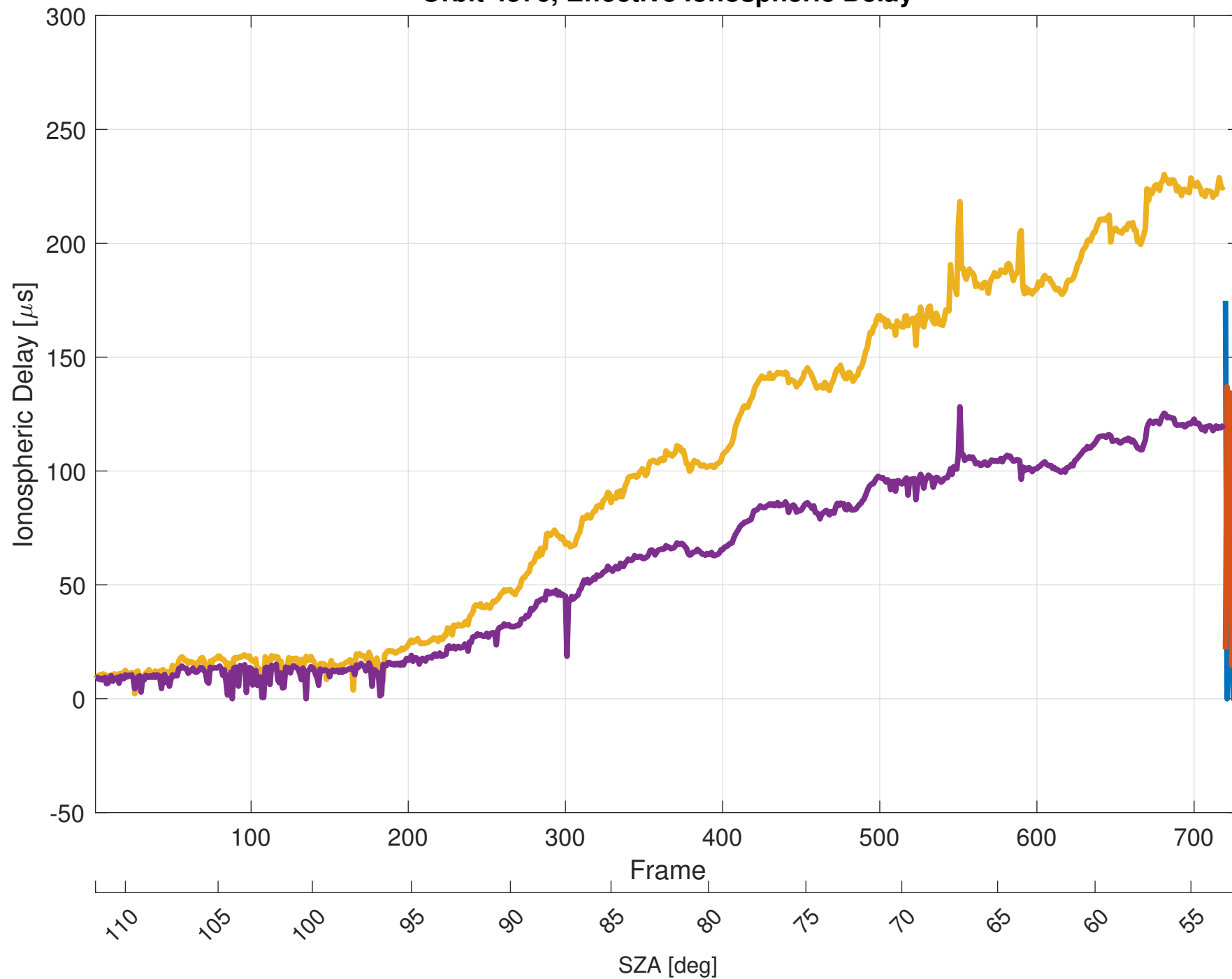
Orbit 4576, Effective Ionospheric Delay
