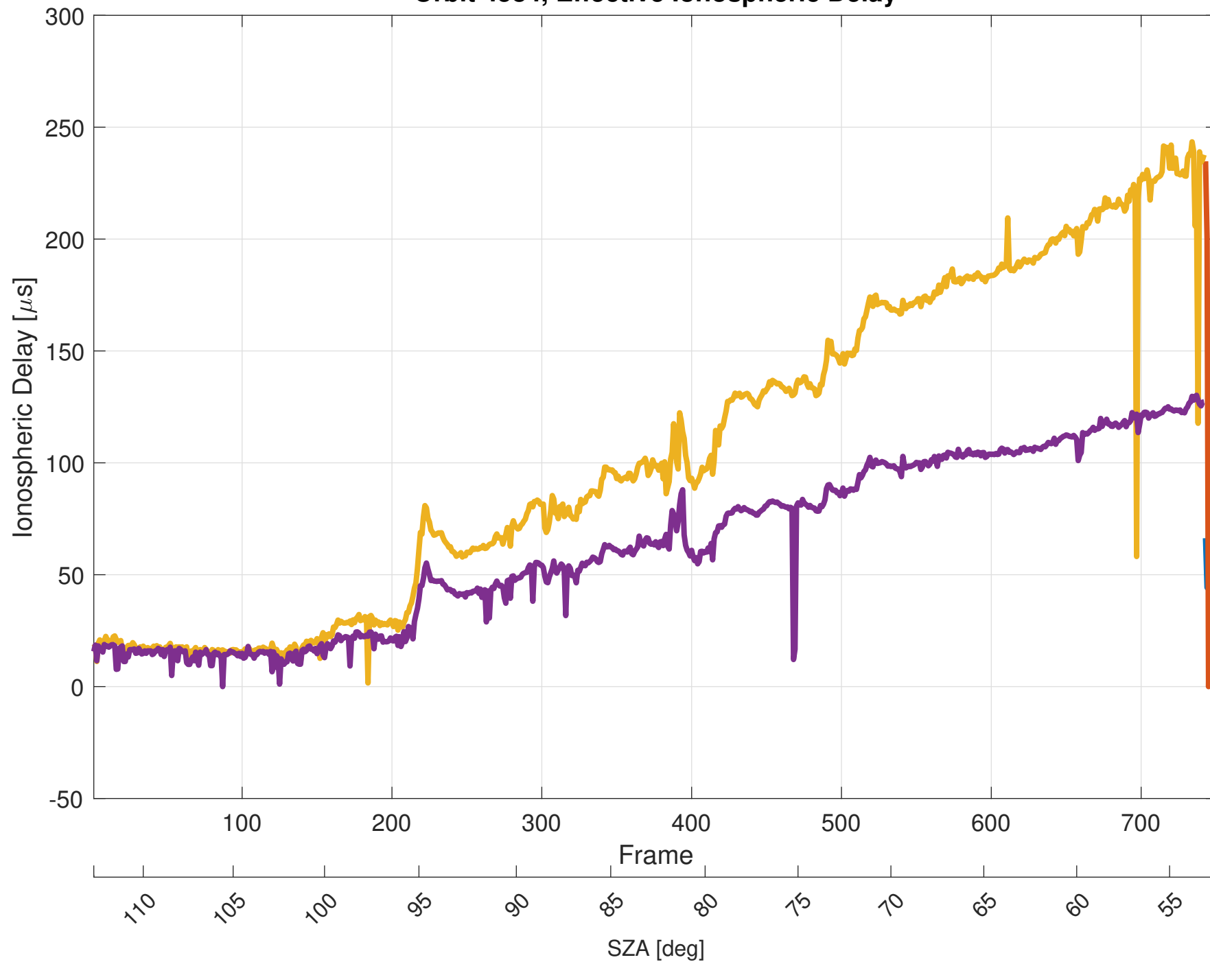
Orbit 4584, Effective Ionospheric Delay
