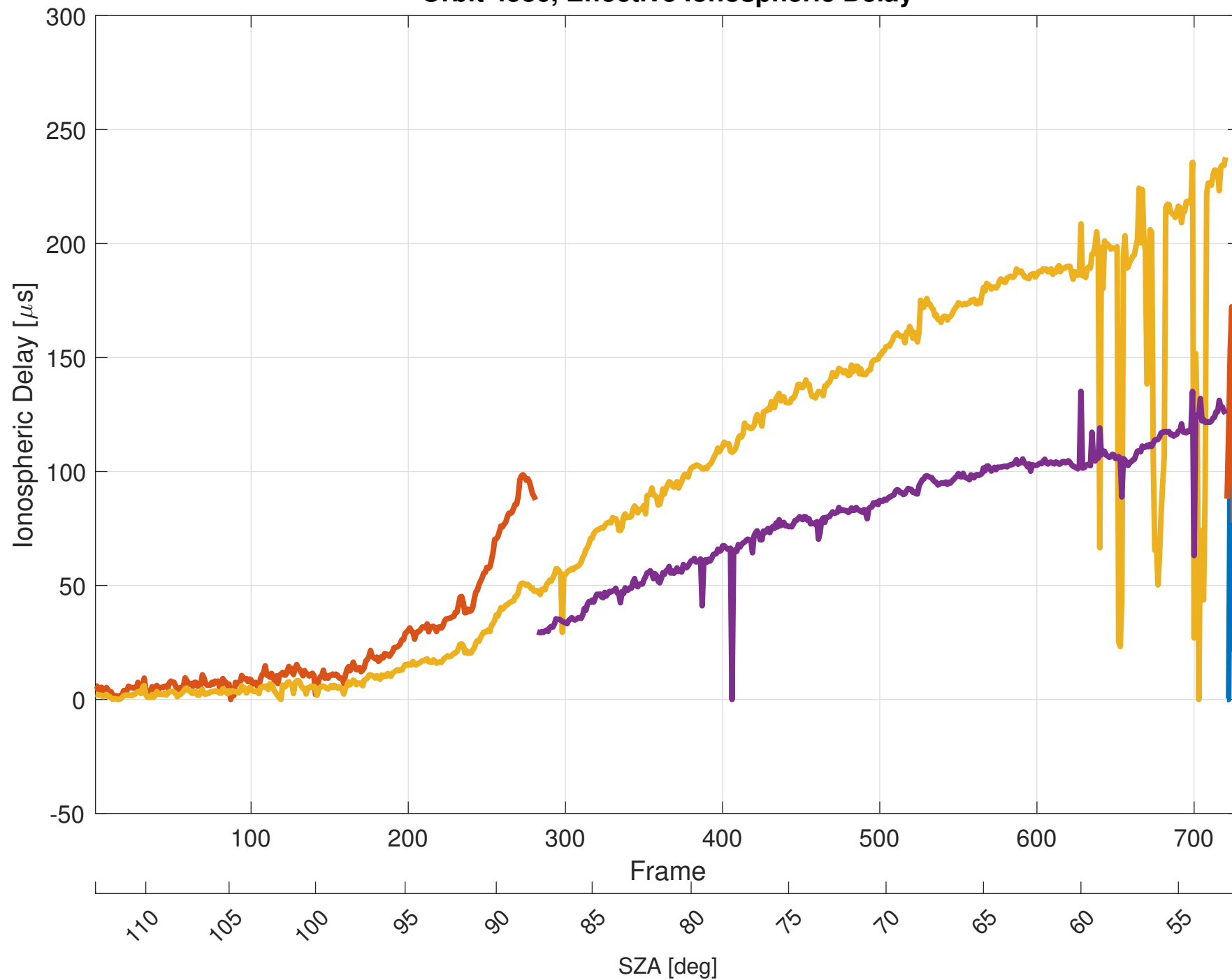
Orbit 4586, Effective Ionospheric Delay
