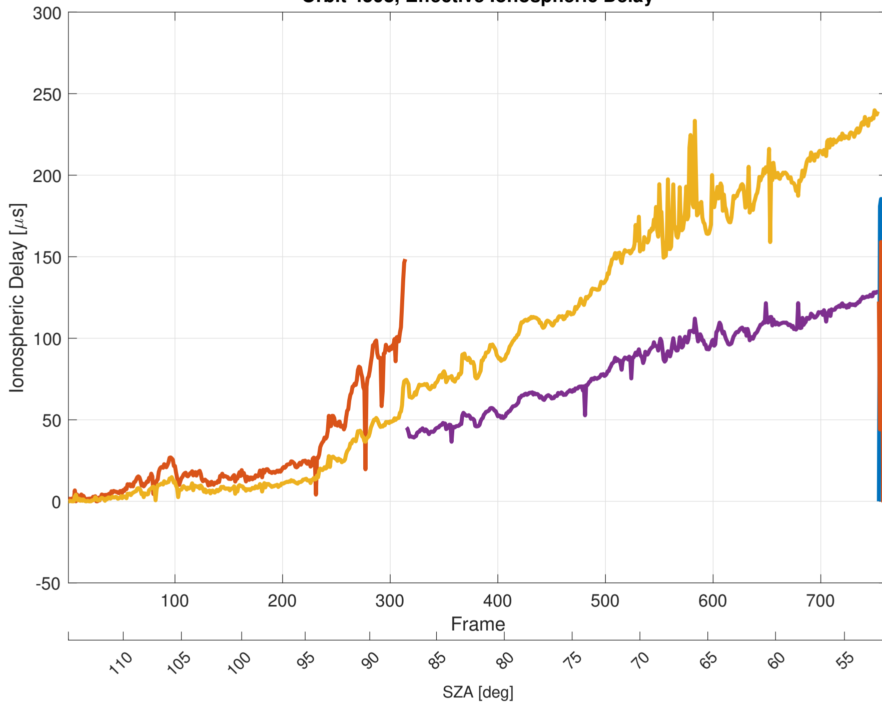
Orbit 4598, Effective Ionospheric Delay
