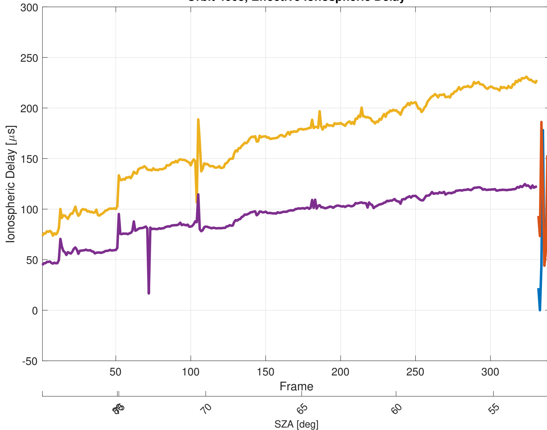
Orbit 4603, Effective Ionospheric Delay
