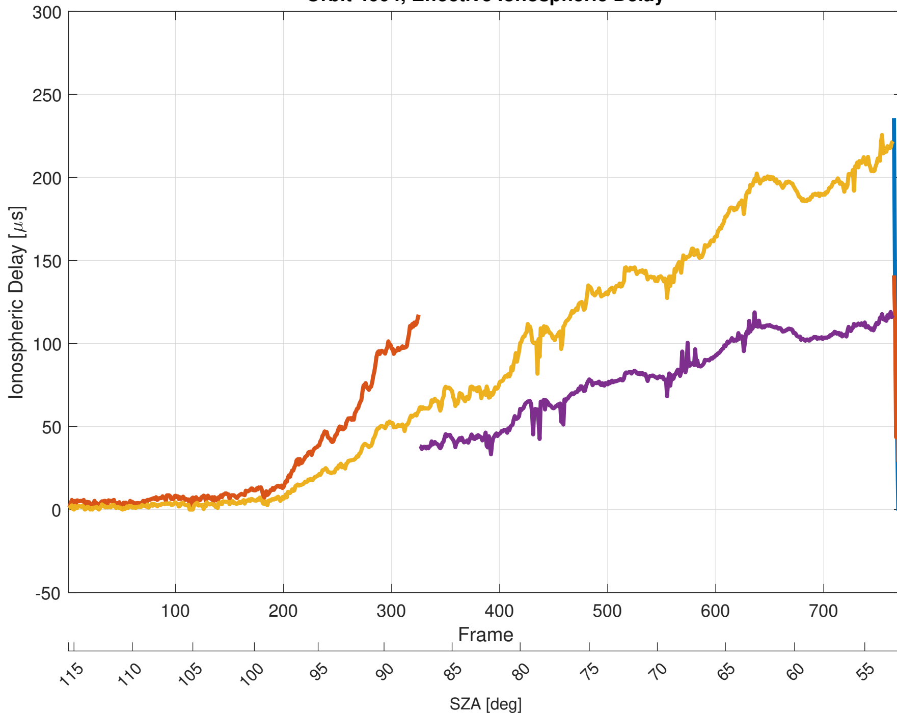
Orbit 4604, Effective Ionospheric Delay
