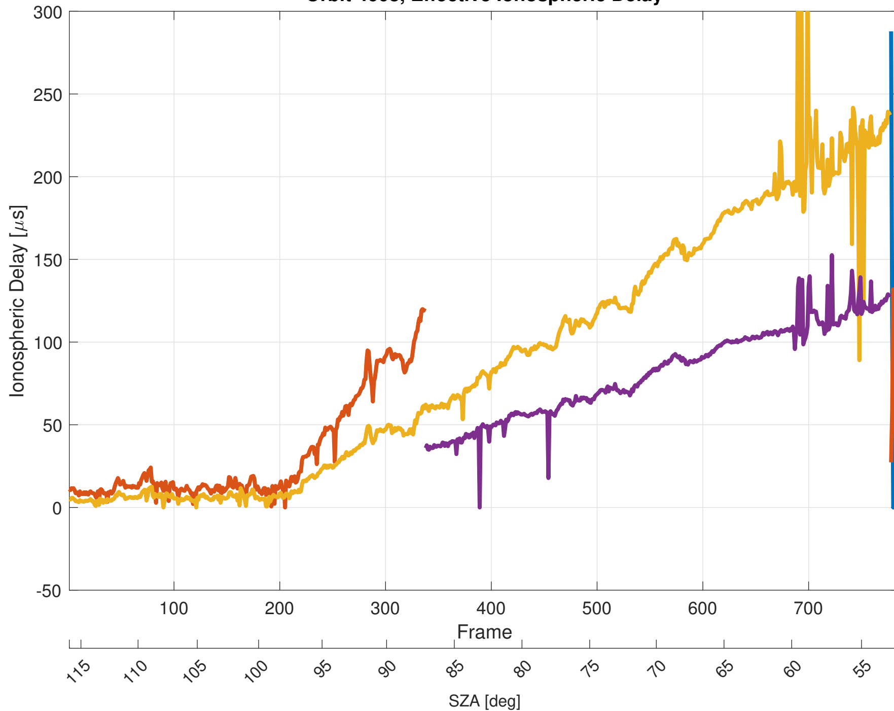
Orbit 4608, Effective Ionospheric Delay
