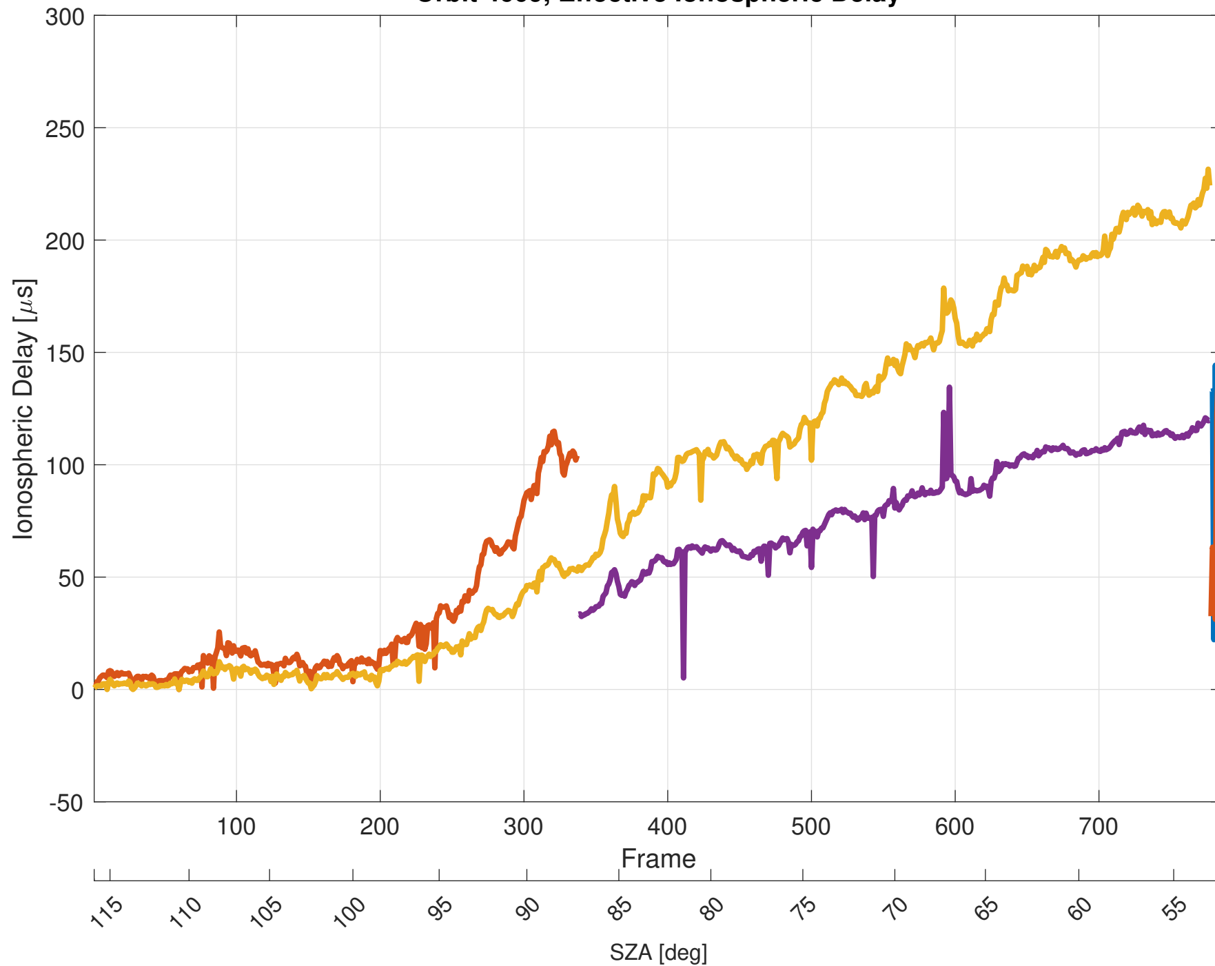
Orbit 4609, Effective Ionospheric Delay
