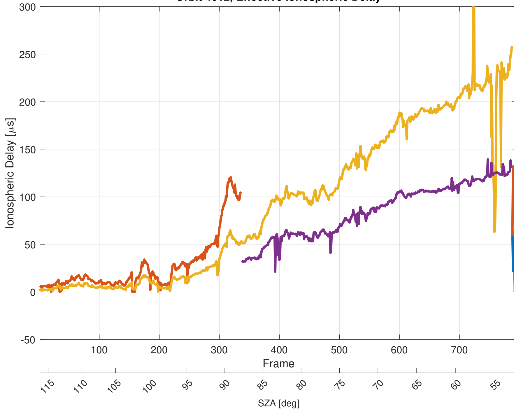
Orbit 4612, Effective Ionospheric Delay
