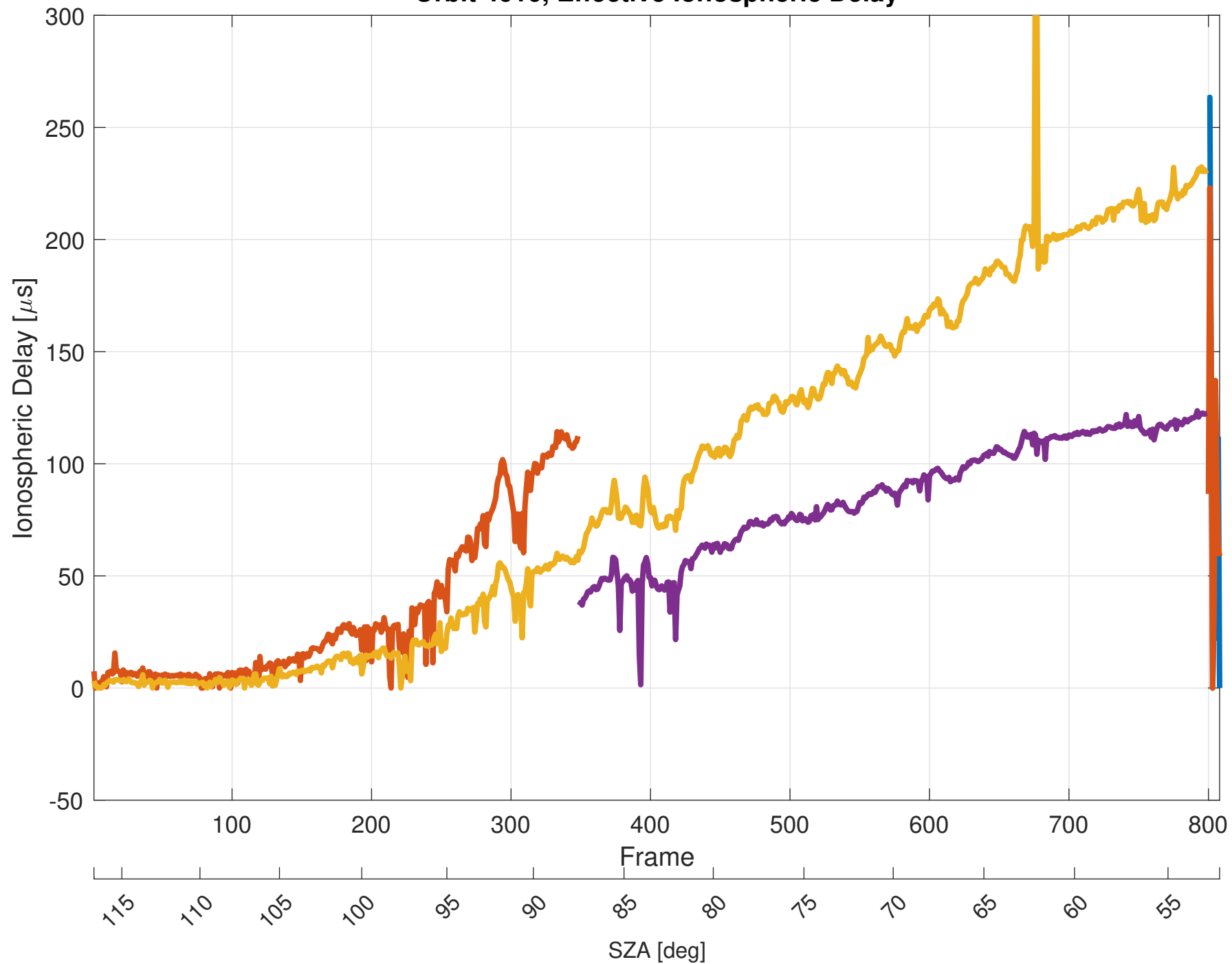
Orbit 4616, Effective Ionospheric Delay
