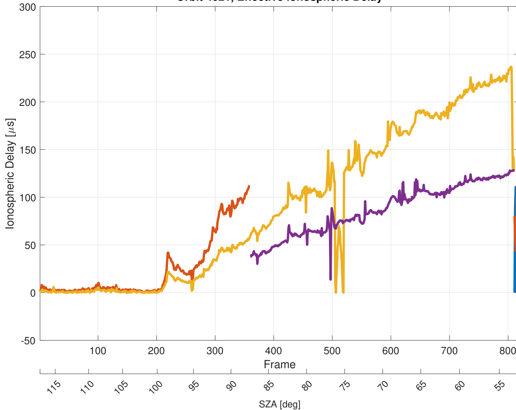
Orbit 4621, Effective Ionospheric Delay
