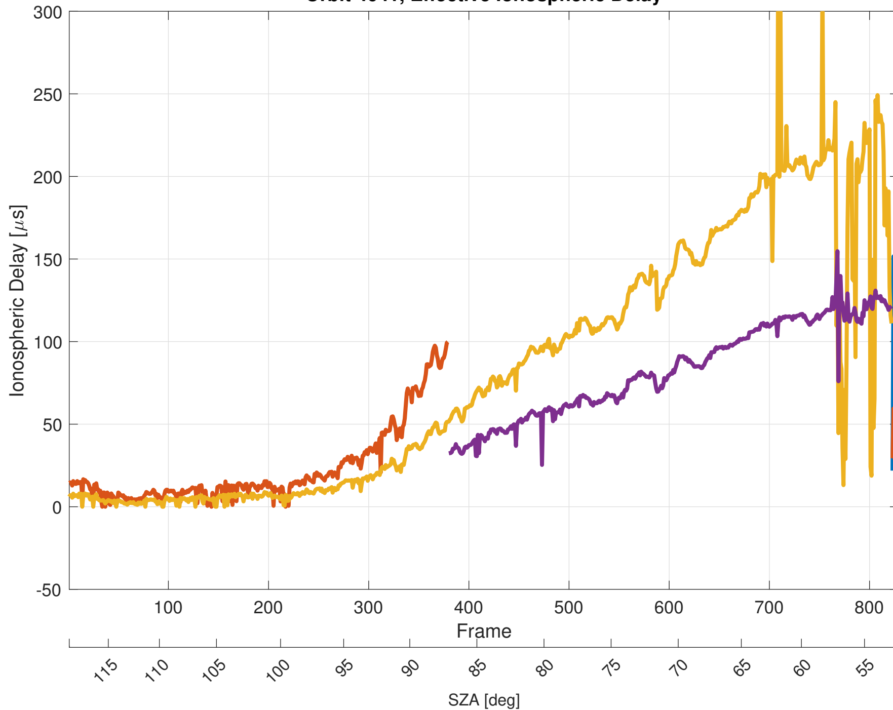
Orbit 4641, Effective Ionospheric Delay
