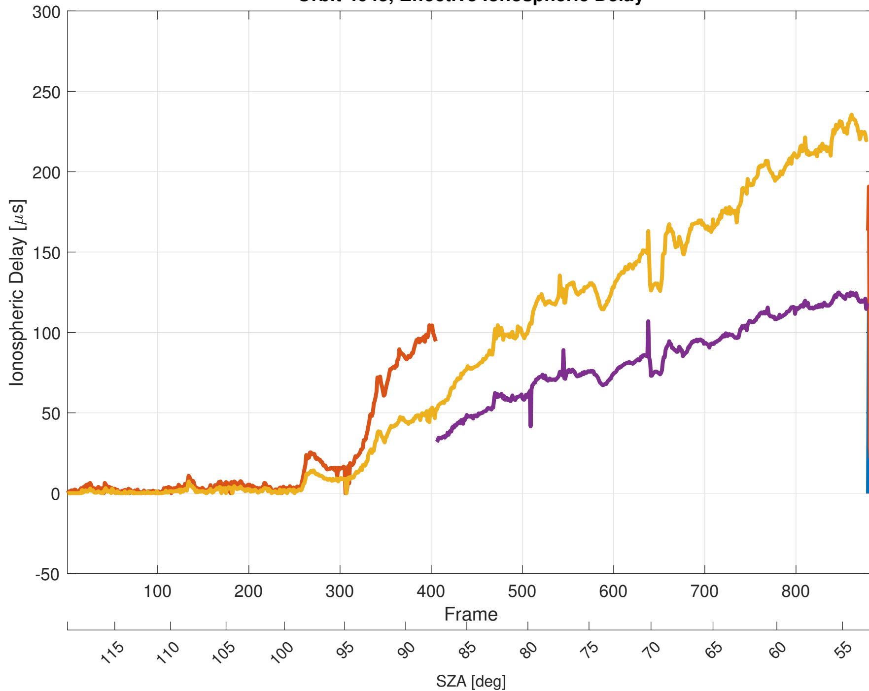
Orbit 4643, Effective Ionospheric Delay
