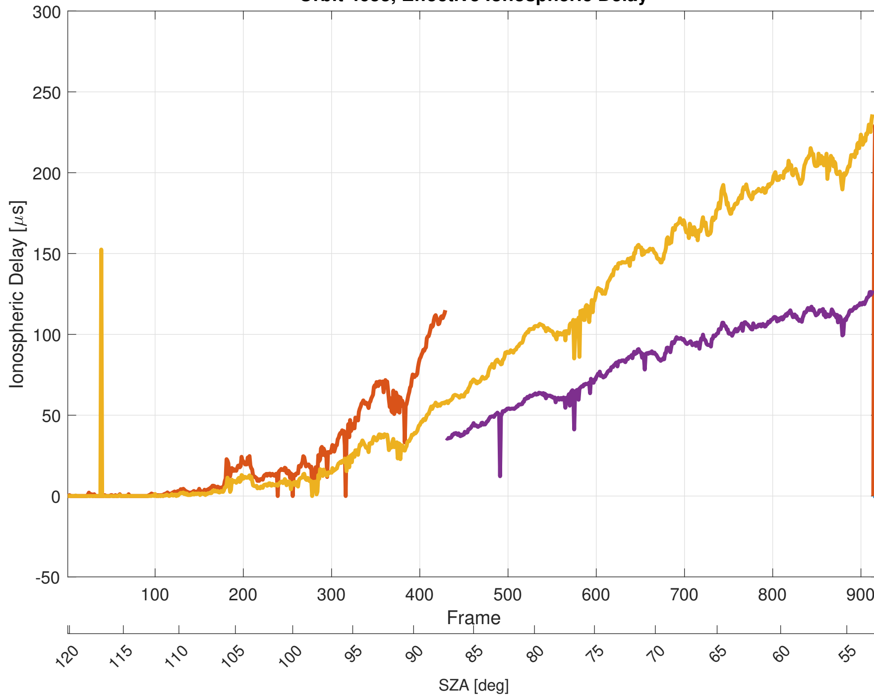
Orbit 4653, Effective Ionospheric Delay
