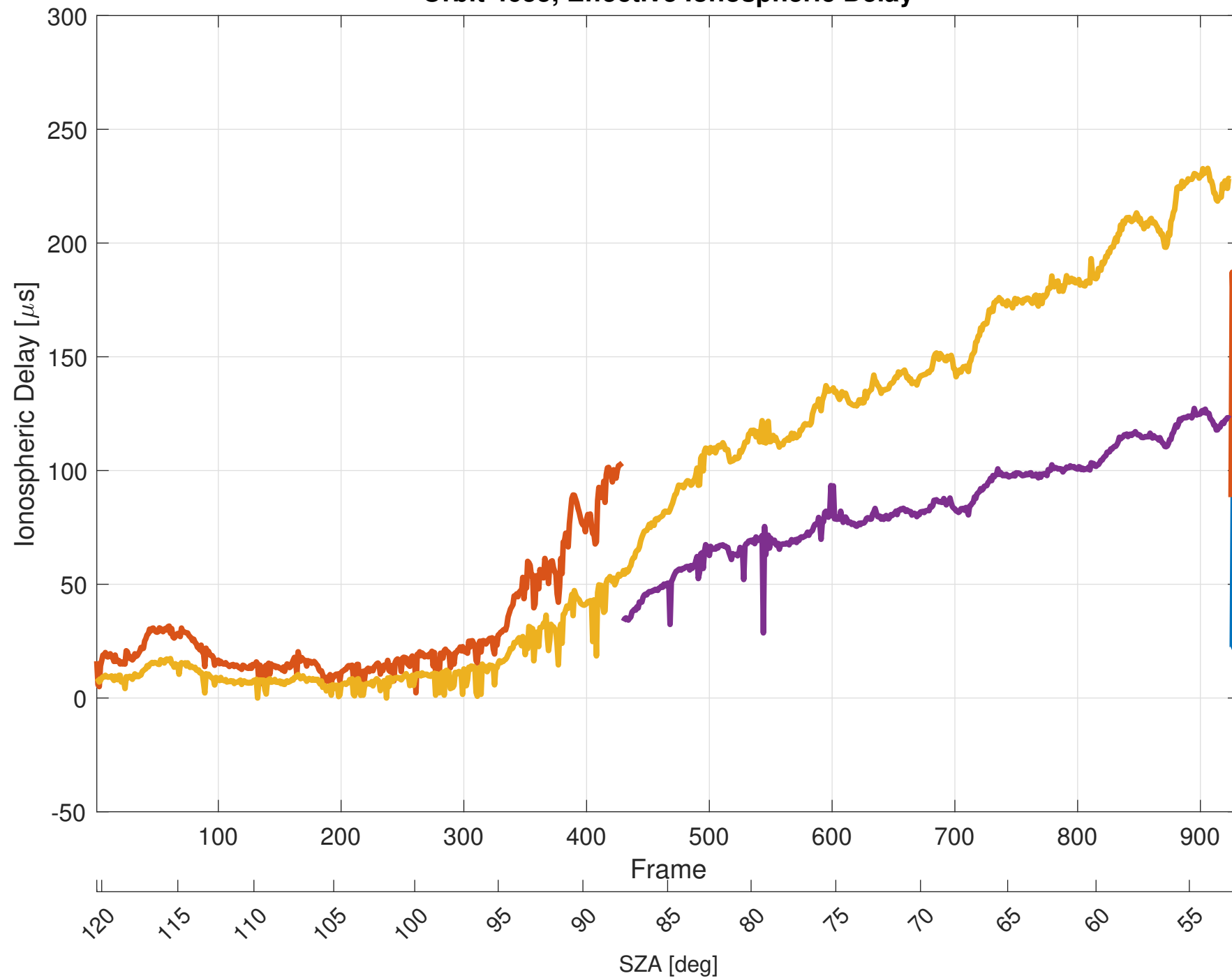
Orbit 4655, Effective Ionospheric Delay
