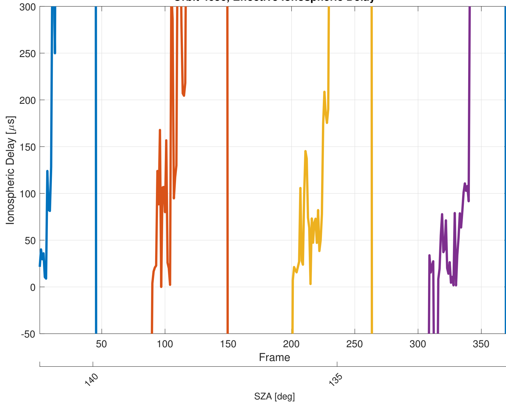
Orbit 4656, Effective Ionospheric Delay
