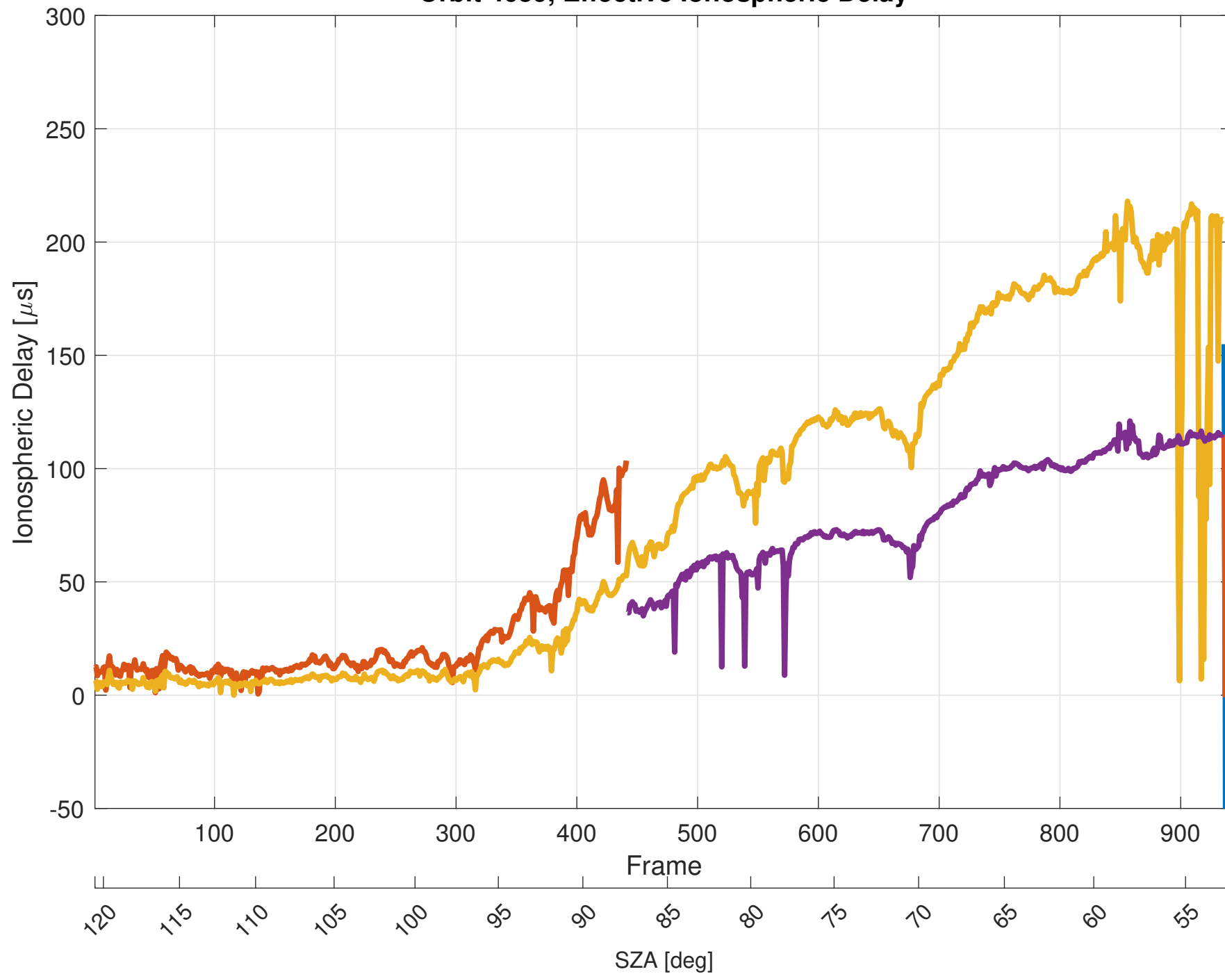
Orbit 4659, Effective Ionospheric Delay
