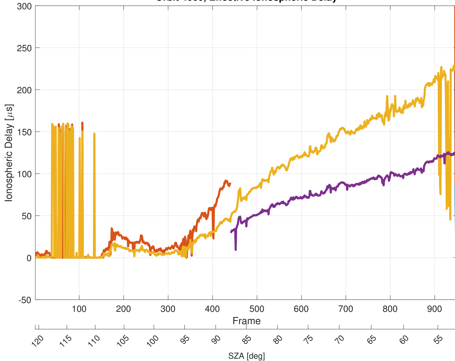
Orbit 4660, Effective Ionospheric Delay
