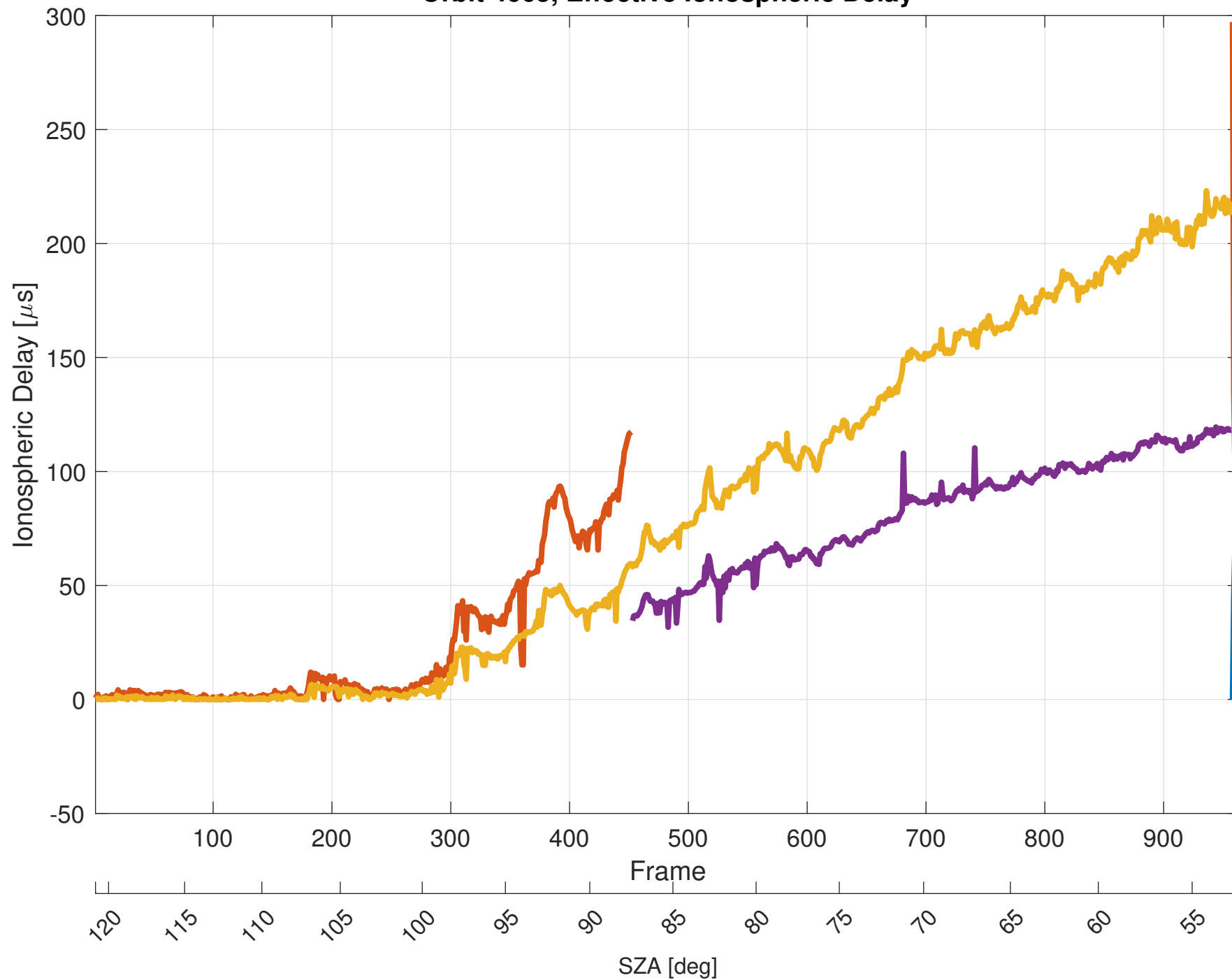
Orbit 4665, Effective Ionospheric Delay
