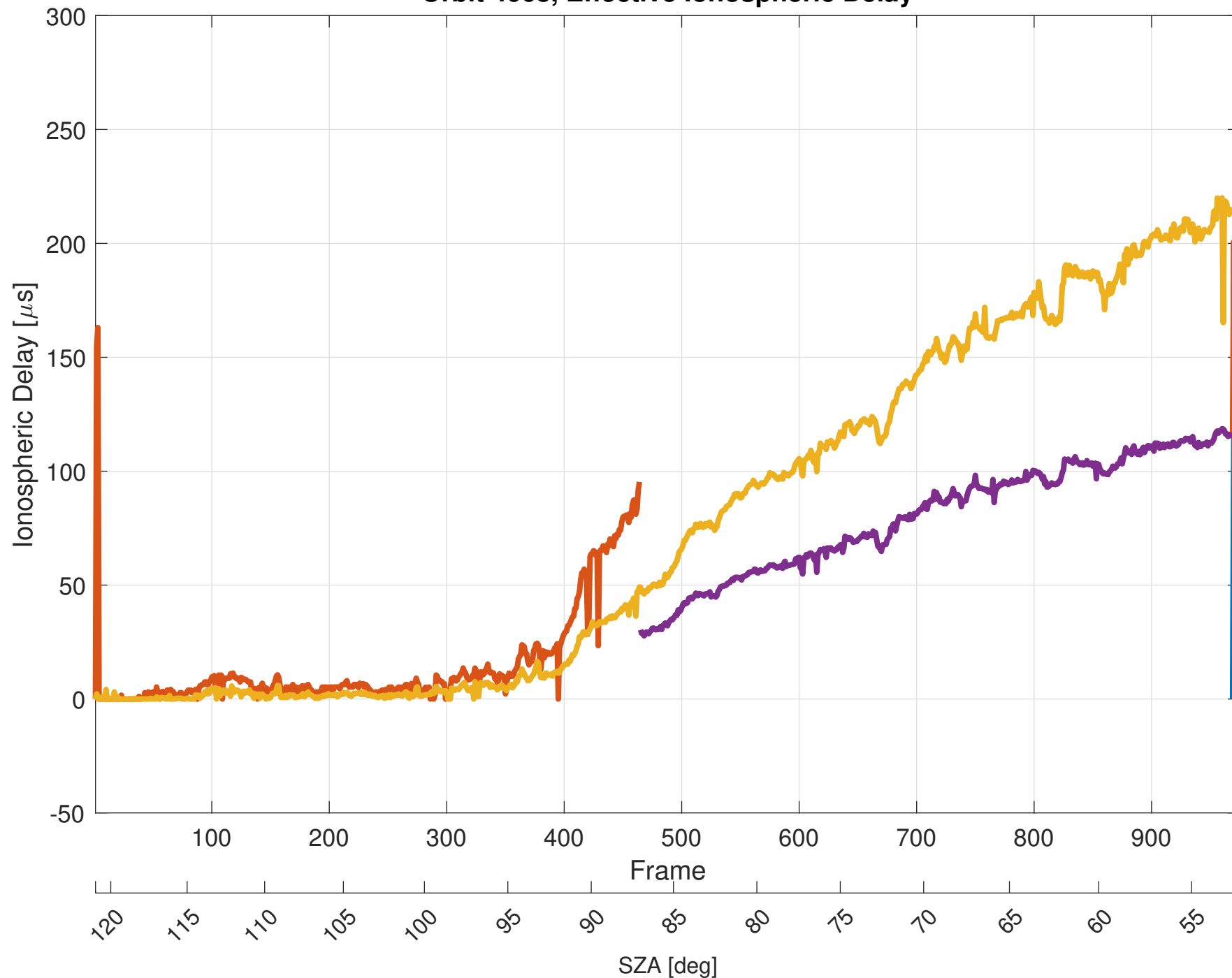
Orbit 4668, Effective Ionospheric Delay
