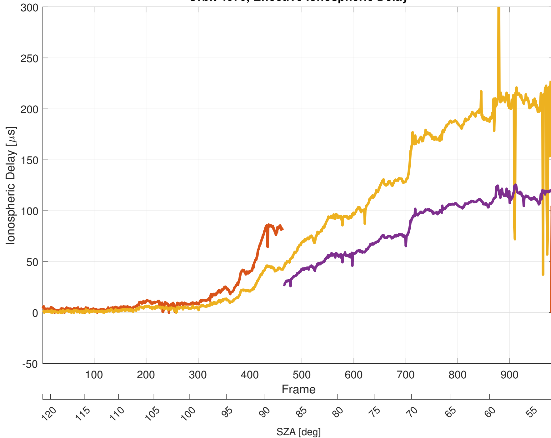
Orbit 4670, Effective Ionospheric Delay
