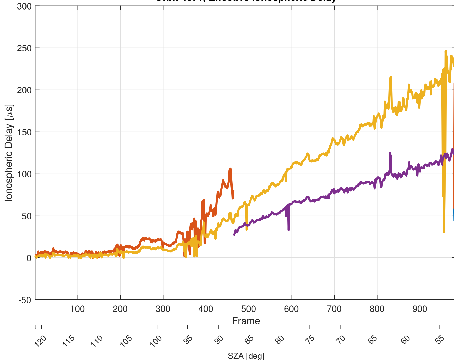
Orbit 4671, Effective Ionospheric Delay
