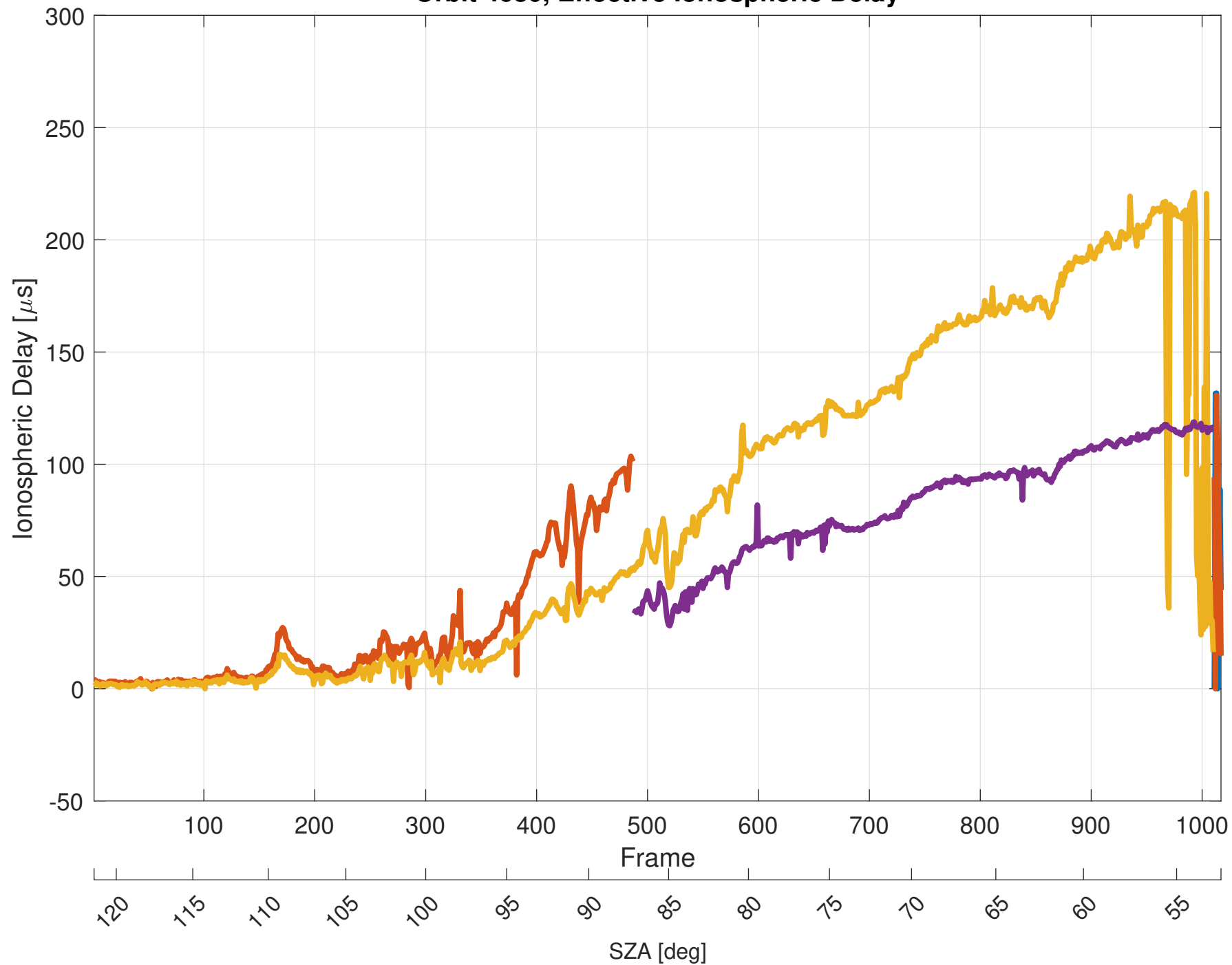
Orbit 4680, Effective Ionospheric Delay
