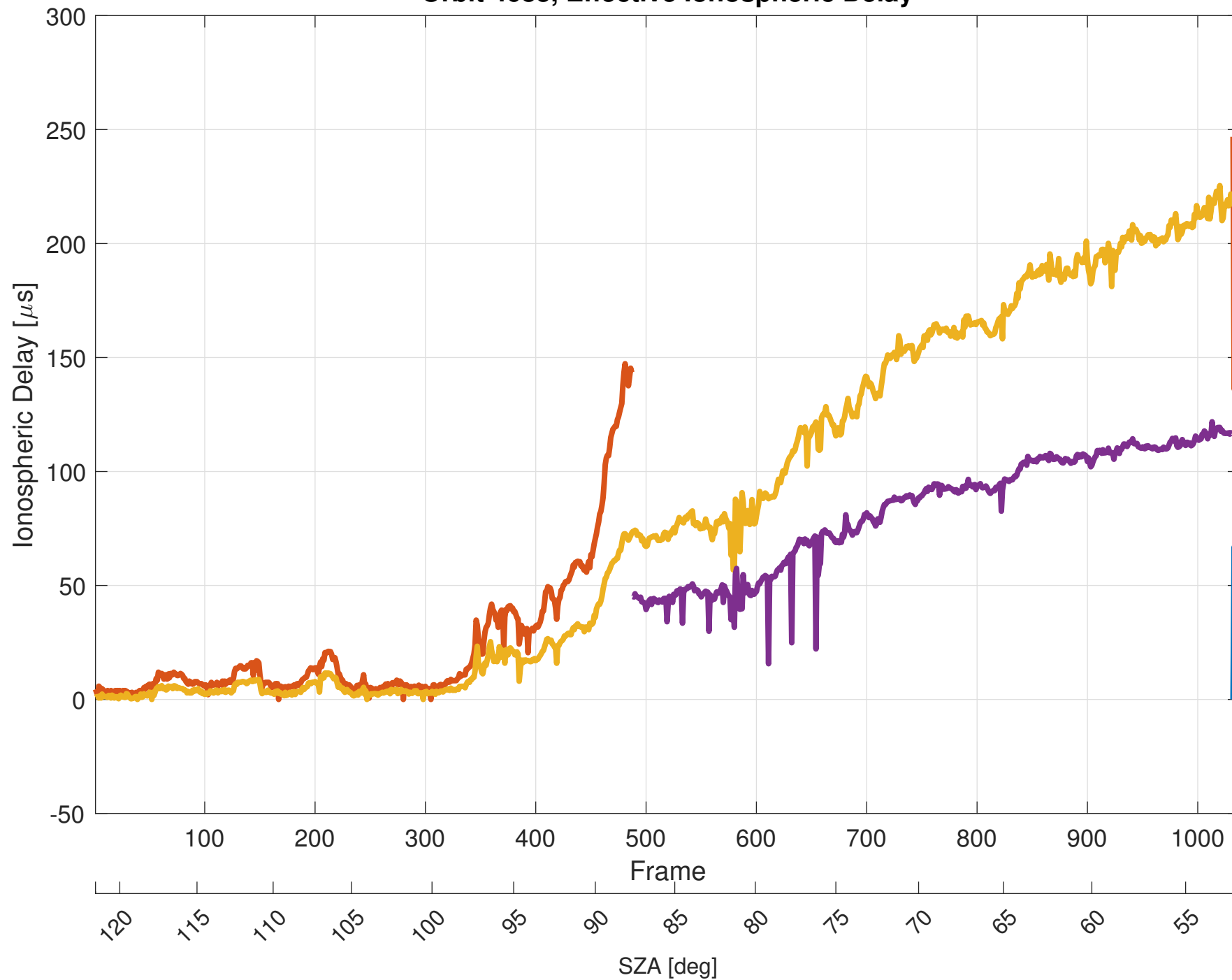
Orbit 4683, Effective Ionospheric Delay
